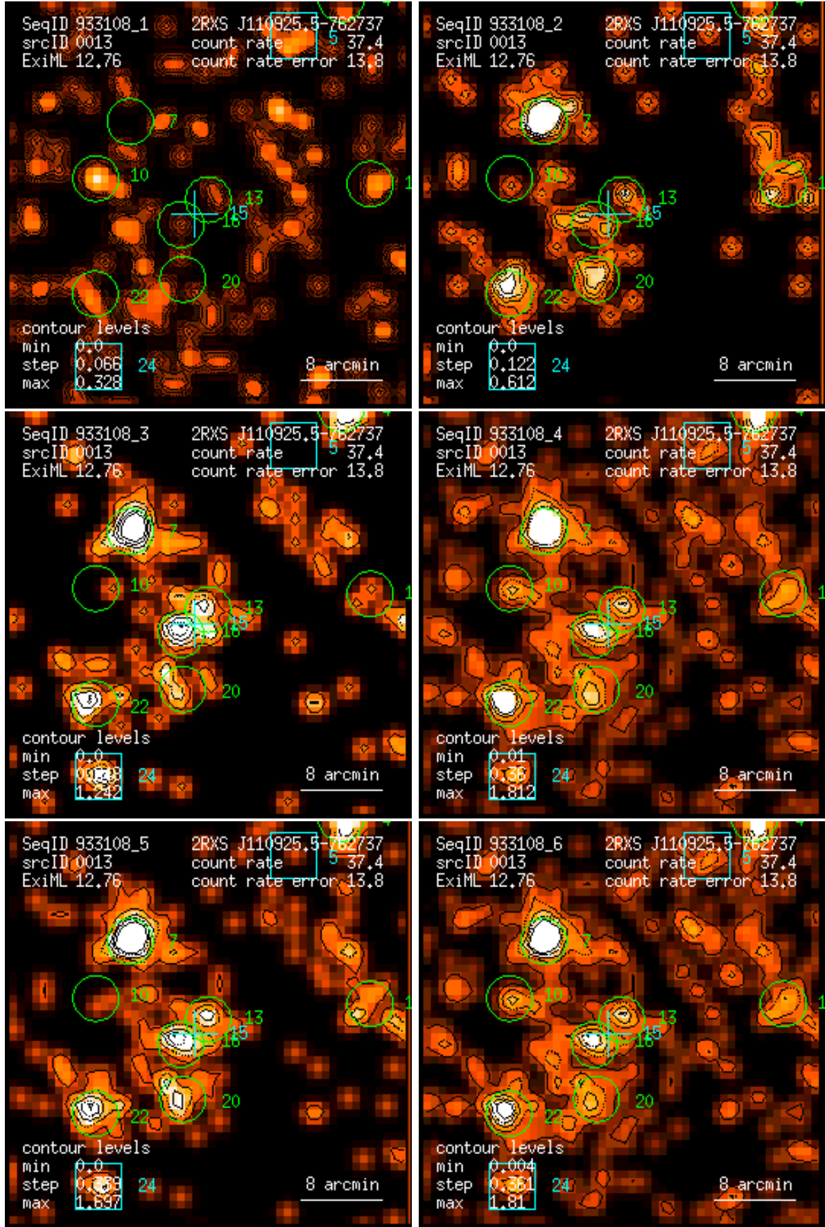
Figure 13: RASS 933108: detection 0013: band rate images, Gaussian filter: (1) PSPC channels 11 – 41, (2) 52 – 90, (3) 91 – 201, (4) 11 – 235, (5) 52 – 201, (6) 11 – 201. Broad band rates in counts/ks. Band rate contour levels in counts/ks/arcmin 2 .
