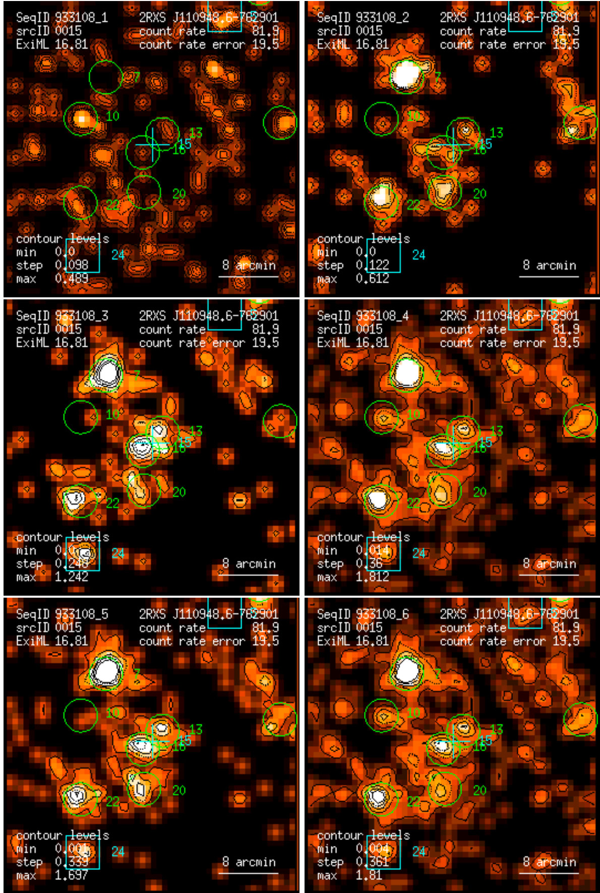
Figure 15: RASS 933108: detection 0015: band rate images, Gaussian filter: (1) PSPC channels 11 – 41, (2) 52 – 90, (3) 91 – 201, (4) 11 – 235, (5) 52 – 201, (6) 11 – 201. Broad band rates in counts/ks. Band rate contour levels in counts/ks/arcmin 2 .
