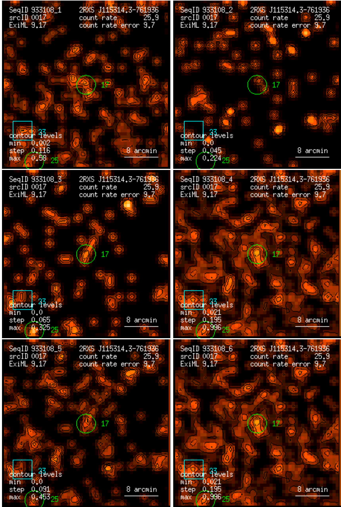
Figure 17: RASS 933108: detection 0017: band rate images, Gaussian filter: (1) PSPC channels 11 – 41, (2) 52 – 90, (3) 91 – 201, (4) 11 – 235, (5) 52 – 201, (6) 11 – 201. Broad band rates in counts/ks. Band rate contour levels in counts/ks/arcmin 2 .
