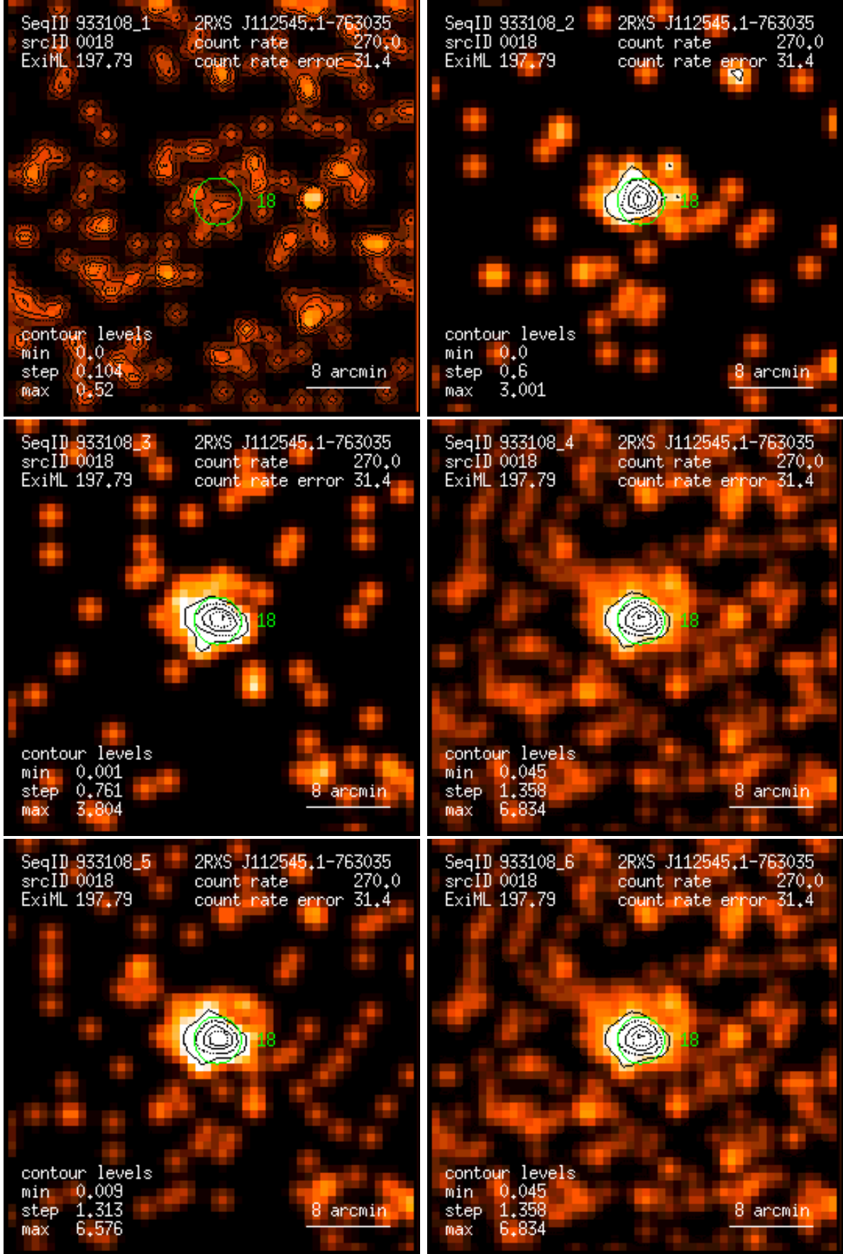
Figure 18: RASS 933108: detection 0018: band rate images, Gaussian filter: (1) PSPC channels 11 – 41, (2) 52 – 90, (3) 91 – 201, (4) 11 – 235, (5) 52 – 201, (6) 11 – 201. Broad band rates in counts/ks. Band rate contour levels in counts/ks/arcmin 2 .
