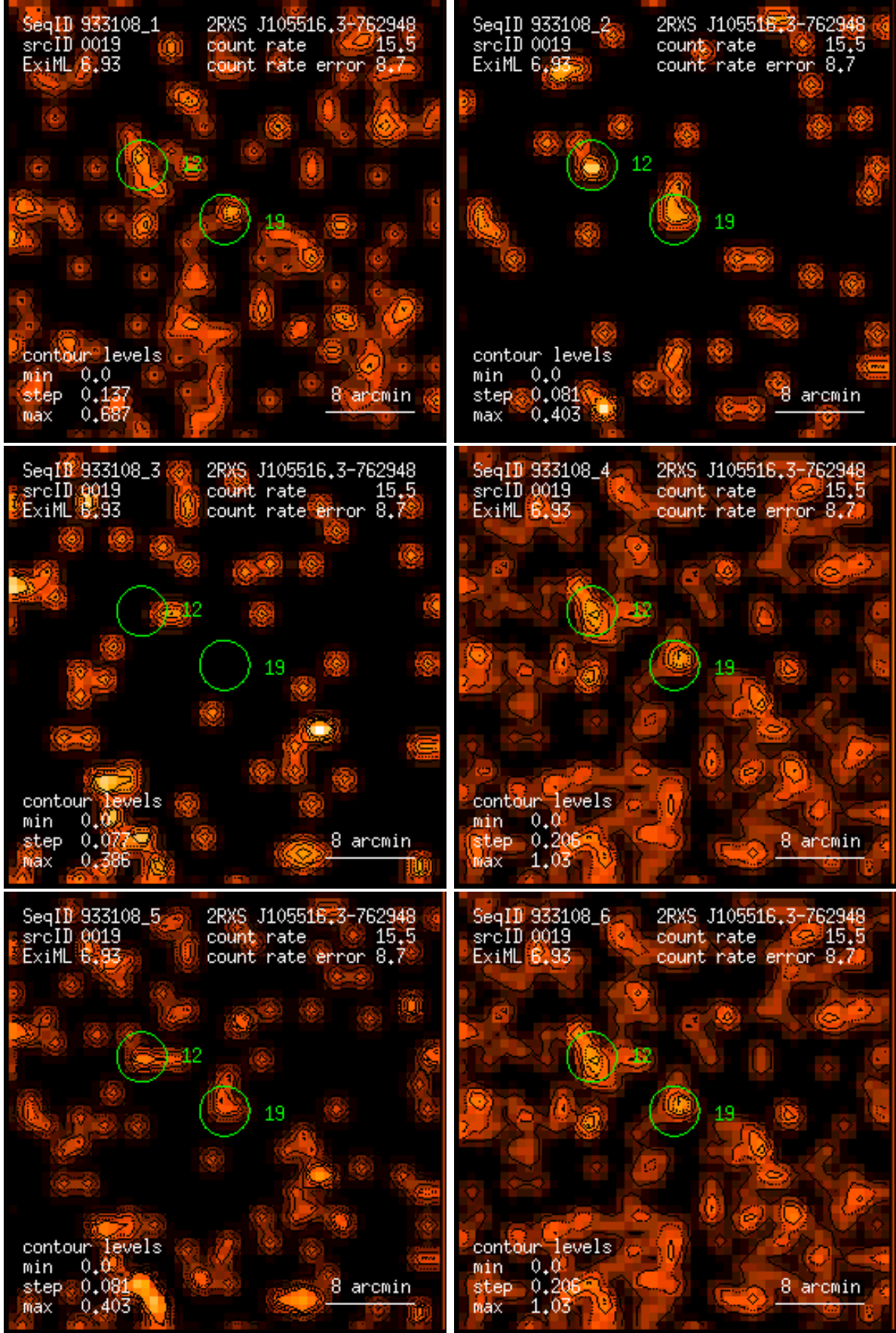
Figure 19: RASS 933108: detection 0019: band rate images, Gaussian filter: (1) PSPC channels 11 – 41, (2) 52 – 90, (3) 91 – 201, (4) 11 – 235, (5) 52 – 201, (6) 11 – 201. Broad band rates in counts/ks. Band rate contour levels in counts/ks/arcmin 2 .
