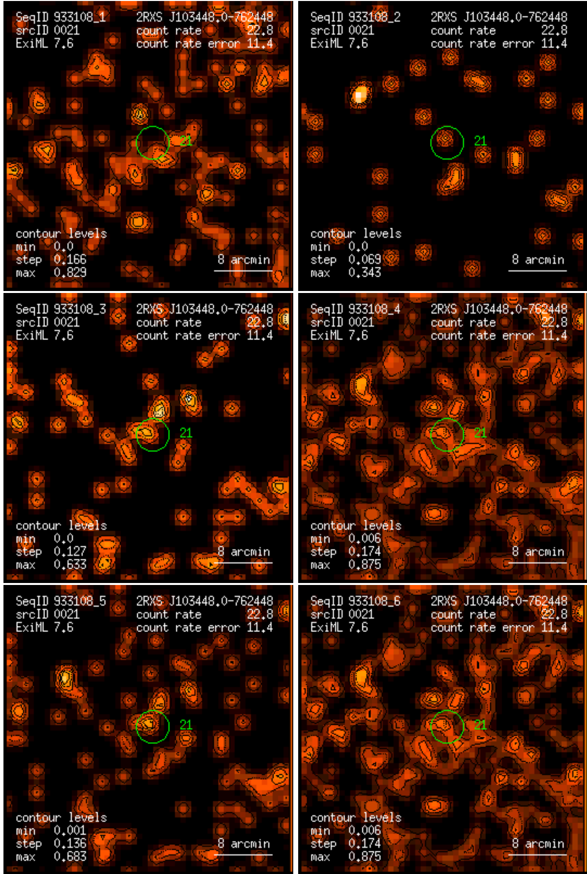
Figure 21: RASS 933108: detection 0021: band rate images, Gaussian filter: (1) PSPC channels 11 – 41, (2) 52 – 90, (3) 91 – 201, (4) 11 – 235, (5) 52 – 201, (6) 11 – 201. Broad band rates in counts/ks. Band rate contour levels in counts/ks/arcmin 2 .
