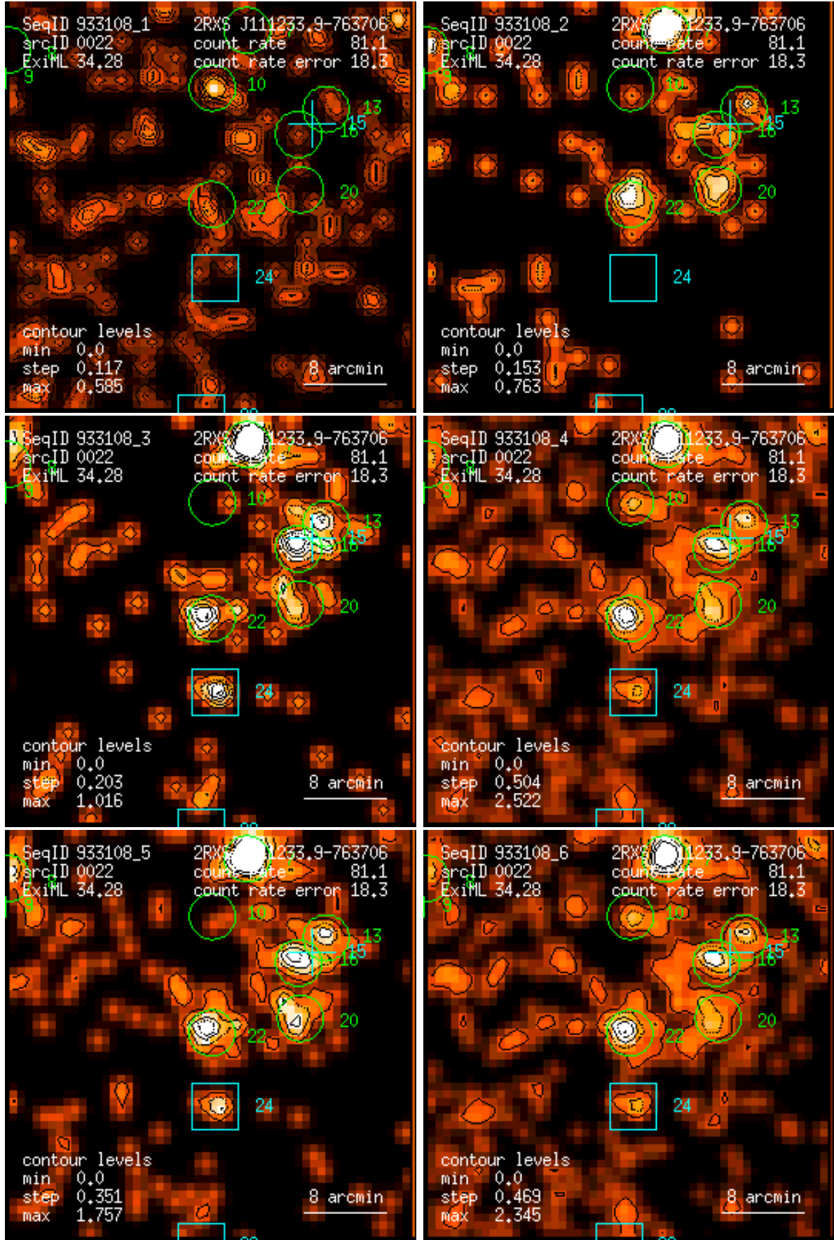
Figure 22: RASS 933108: detection 0022: band rate images, Gaussian filter: (1) PSPC channels 11 – 41, (2) 52 – 90, (3) 91 – 201, (4) 11 – 235, (5) 52 – 201, (6) 11 – 201. Broad band rates in counts/ks. Band rate contour levels in counts/ks/arcmin 2 .
