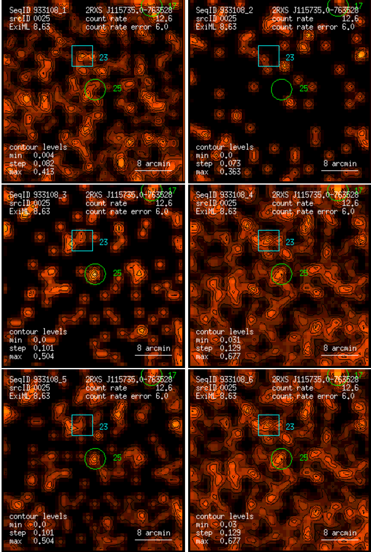
Figure 25: RASS 933108: detection 0025: band rate images, Gaussian filter: (1) PSPC channels 11 – 41, (2) 52 – 90, (3) 91 – 201, (4) 11 – 235, (5) 52 – 201, (6) 11 – 201. Broad band rates in counts/ks. Band rate contour levels in counts/ks/arcmin 2 .
