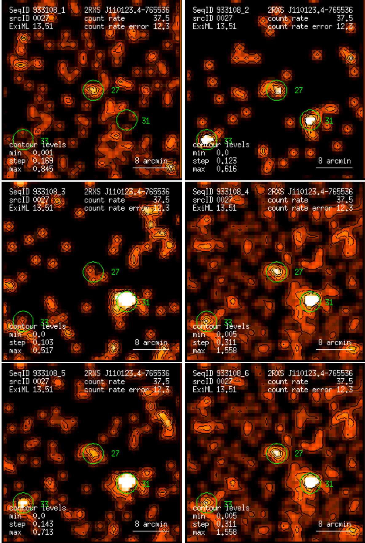
Figure 27: RASS 933108: detection 0027: band rate images, Gaussian filter: (1) PSPC channels 11 – 41, (2) 52 – 90, (3) 91 – 201, (4) 11 – 235, (5) 52 – 201, (6) 11 – 201. Broad band rates in counts/ks. Band rate contour levels in counts/ks/arcmin 2 .
