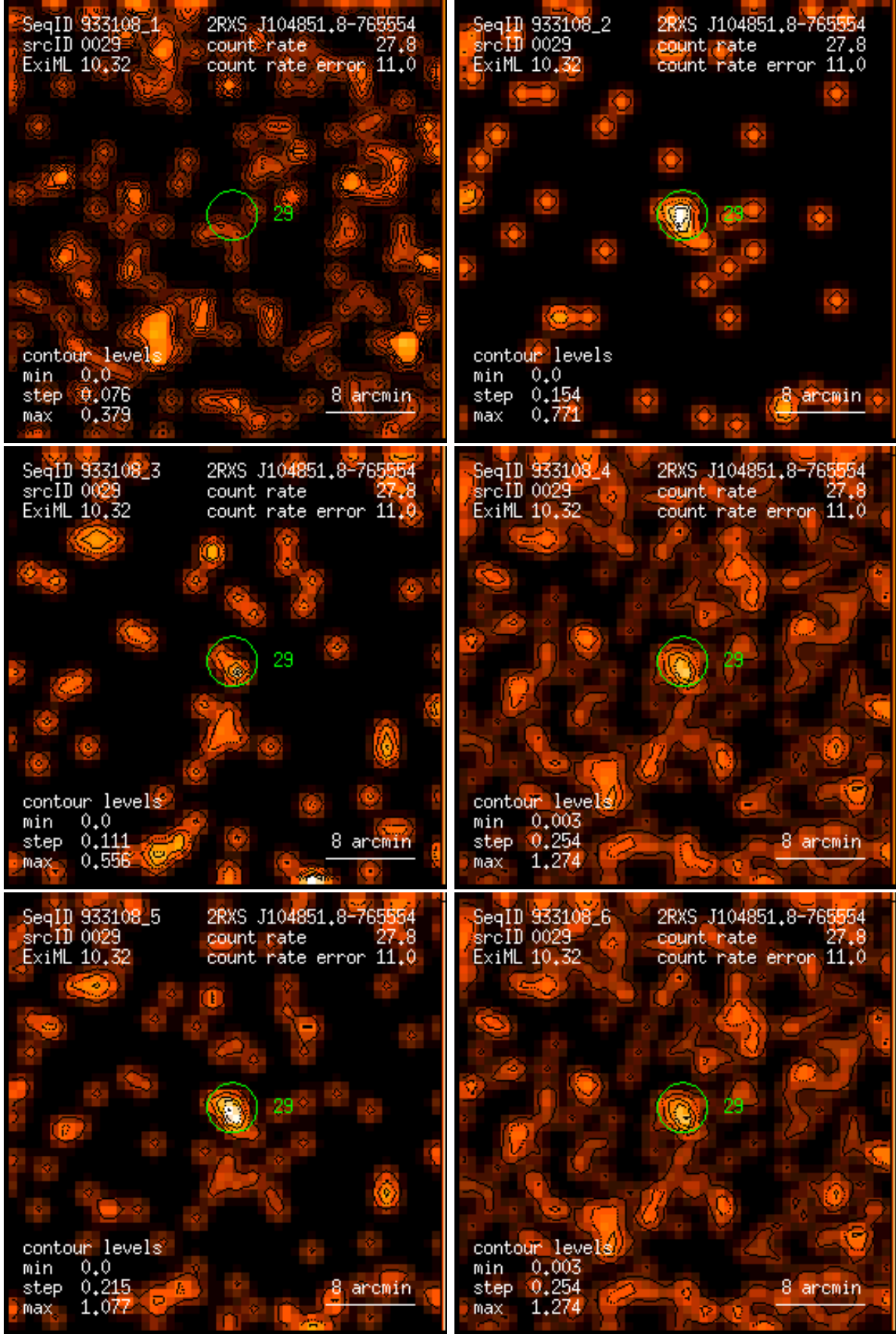
Figure 29: RASS 933108: detection 0029: band rate images, Gaussian filter: (1) PSPC channels 11 – 41, (2) 52 – 90, (3) 91 – 201, (4) 11 – 235, (5) 52 – 201, (6) 11 – 201. Broad band rates in counts/ks. Band rate contour levels in counts/ks/arcmin 2 .
