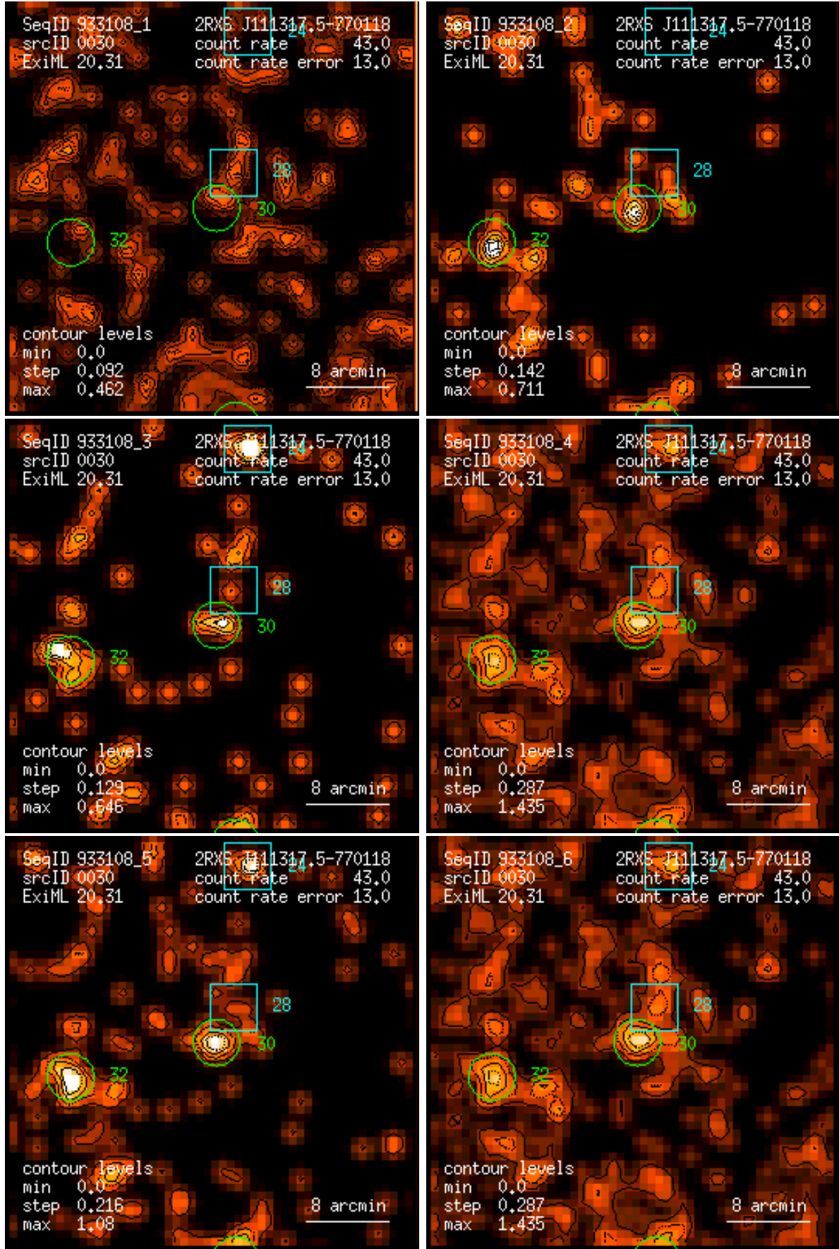
Figure 30: RASS 933108: detection 0030: band rate images, Gaussian filter: (1) PSPC channels 11 – 41, (2) 52 – 90, (3) 91 – 201, (4) 11 – 235, (5) 52 – 201, (6) 11 – 201. Broad band rates in counts/ks. Band rate contour levels in counts/ks/arcmin 2 .
