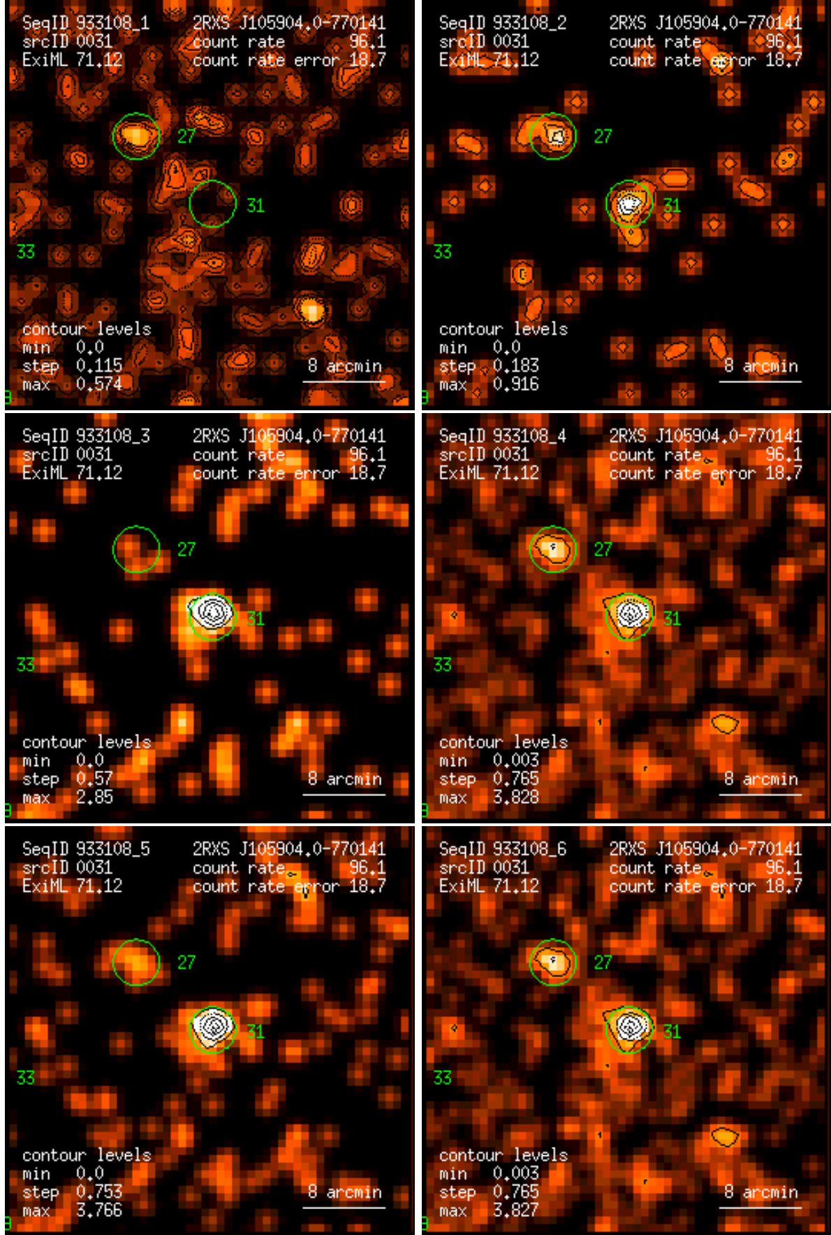
Figure 31: RASS 933108: detection 0031: band rate images, Gaussian filter: (1) PSPC channels 11 – 41, (2) 52 – 90, (3) 91 – 201, (4) 11 – 235, (5) 52 – 201, (6) 11 – 201. Broad band rates in counts/ks. Band rate contour levels in counts/ks/arcmin 2 .
