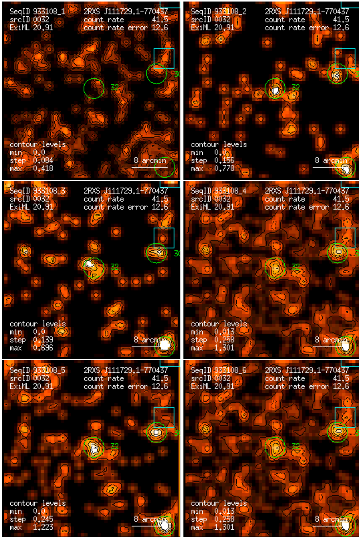
Figure 32: RASS 933108: detection 0032: band rate images, Gaussian filter: (1) PSPC channels 11 – 41, (2) 52 – 90, (3) 91 – 201, (4) 11 – 235, (5) 52 – 201, (6) 11 – 201. Broad band rates in counts/ks. Band rate contour levels in counts/ks/arcmin 2 .
