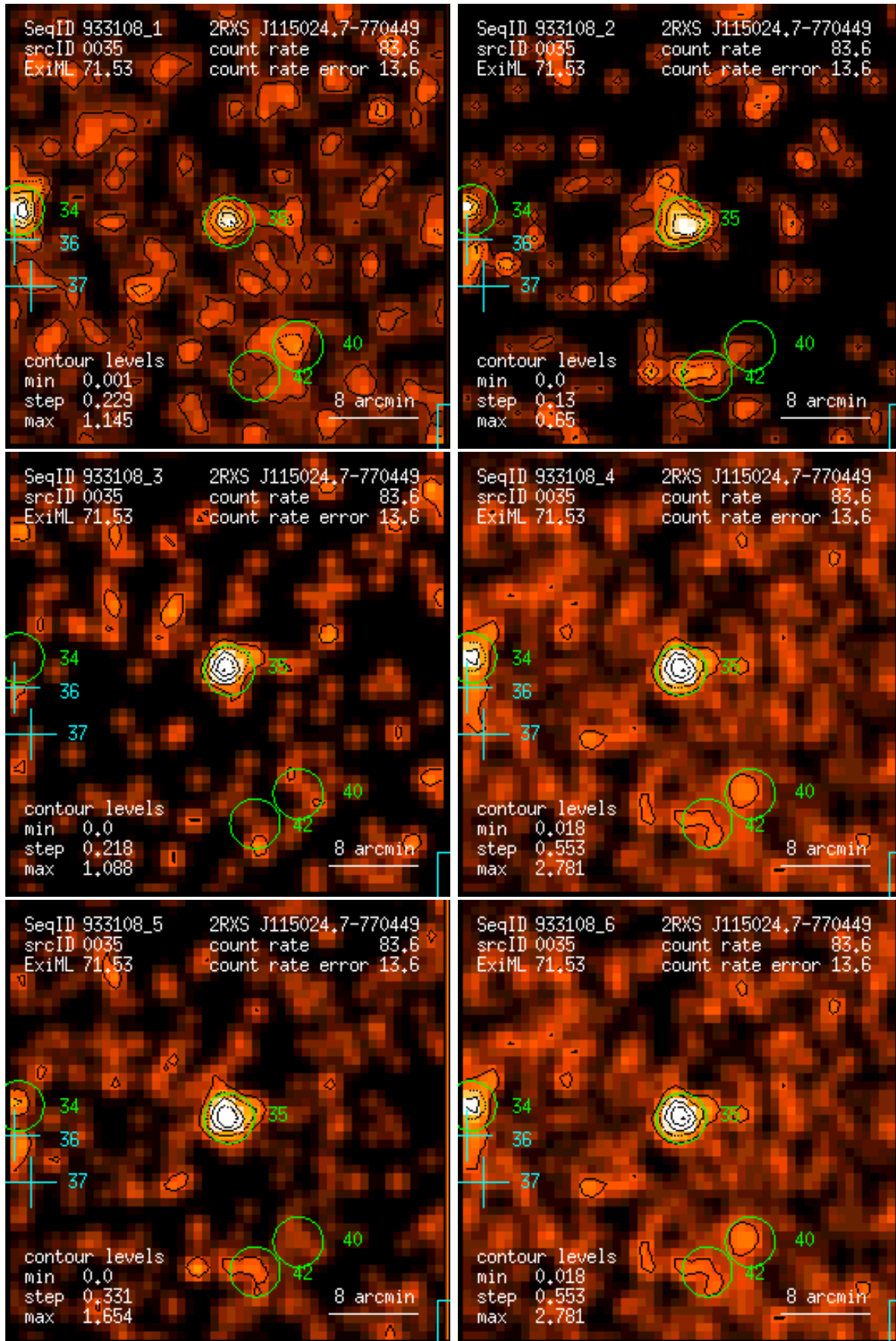
Figure 35: RASS 933108: detection 0035: band rate images, Gaussian filter: (1) PSPC channels 11 – 41, (2) 52 – 90, (3) 91 – 201, (4) 11 – 235, (5) 52 – 201, (6) 11 – 201. Broad band rates in counts/ks. Band rate contour levels in counts/ks/arcmin 2 .
