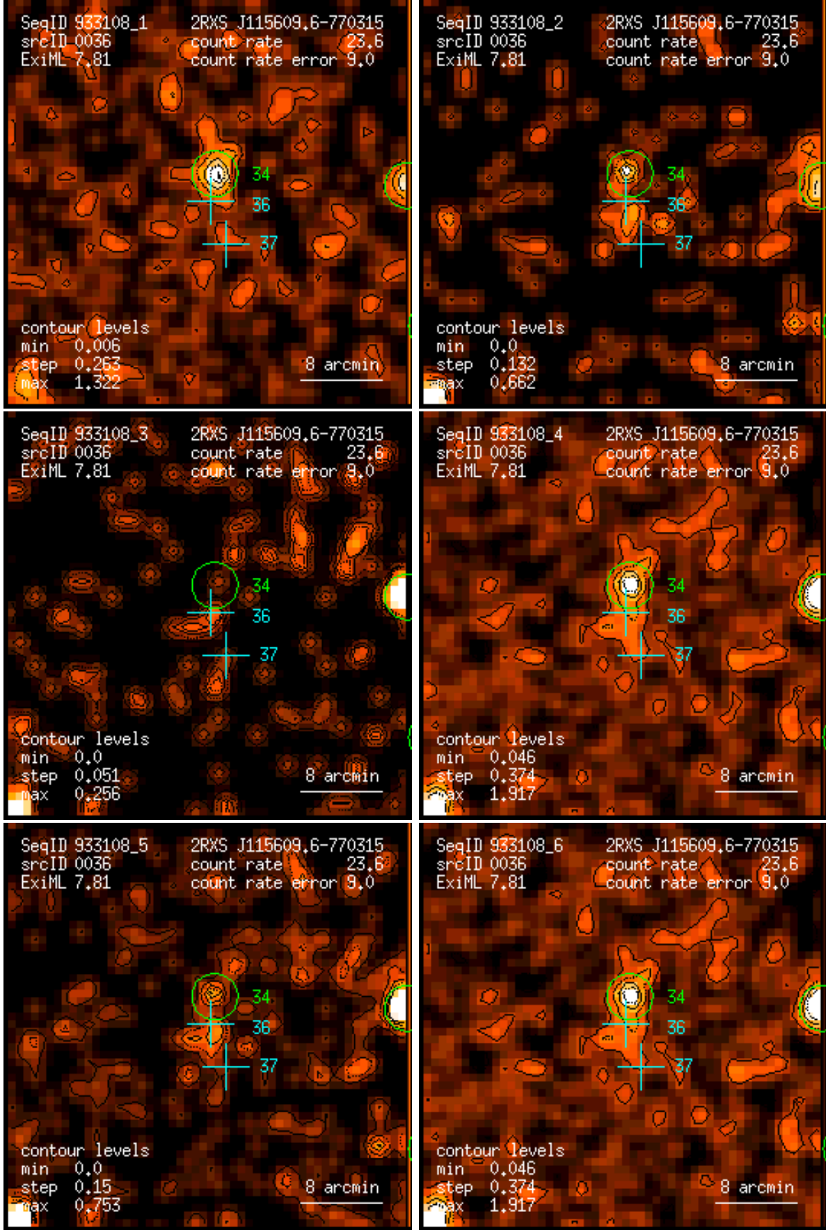
Figure 36: RASS 933108: detection 0036: band rate images, Gaussian filter: (1) PSPC channels 11 – 41, (2) 52 – 90, (3) 91 – 201, (4) 11 – 235, (5) 52 – 201, (6) 11 – 201. Broad band rates in counts/ks. Band rate contour levels in counts/ks/arcmin 2 .
