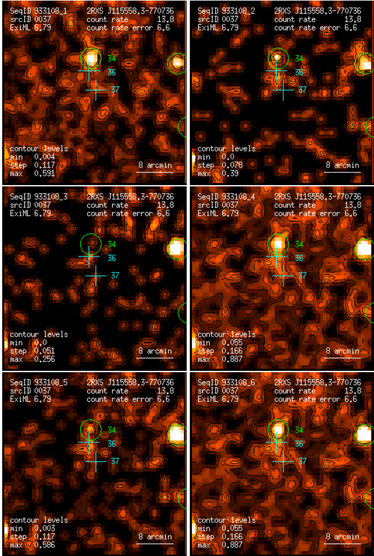
Figure 37: RASS 933108: detection 0037: band rate images, Gaussian filter: (1) PSPC channels 11 – 41, (2) 52 – 90, (3) 91 – 201, (4) 11 – 235, (5) 52 – 201, (6) 11 – 201. Broad band rates in counts/ks. Band rate contour levels in counts/ks/arcmin 2 .
