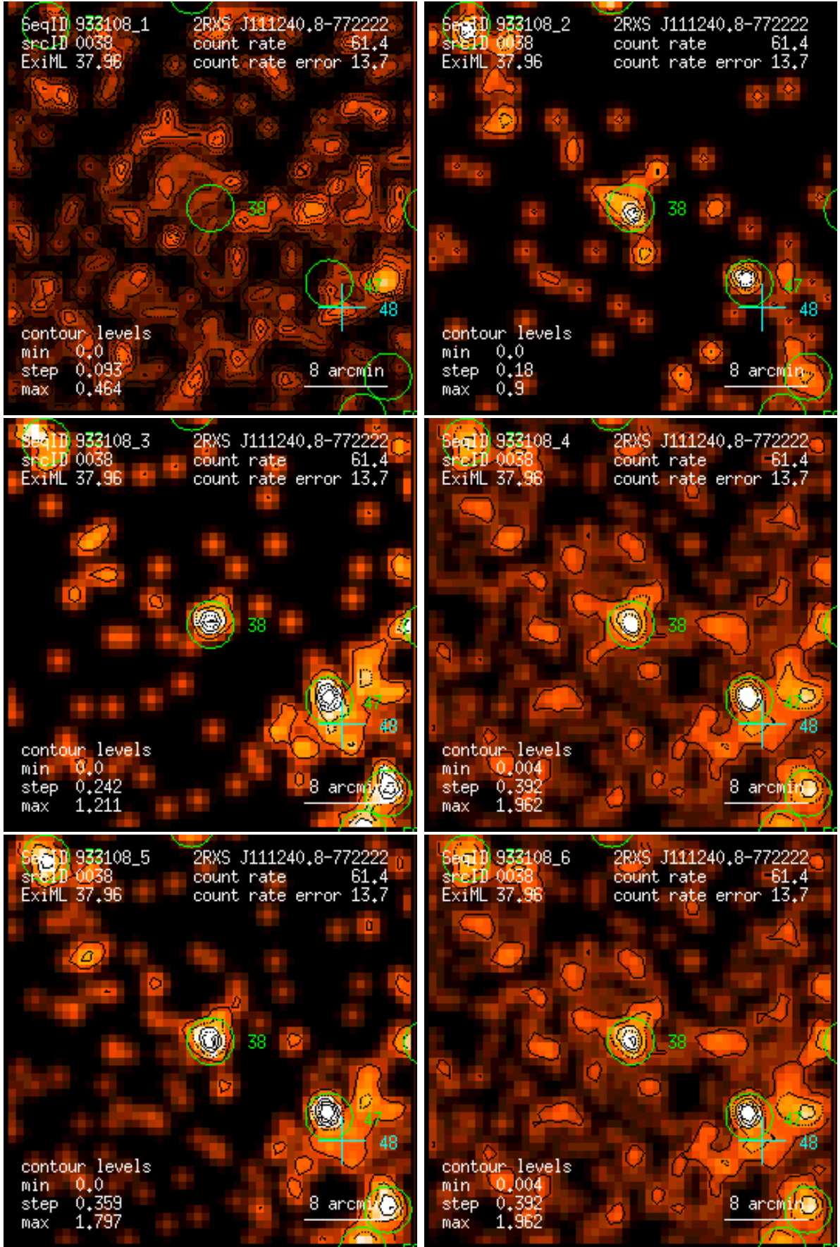
Figure 38: RASS 933108: detection 0038: band rate images, Gaussian filter: (1) PSPC channels 11 – 41, (2) 52 – 90, (3) 91 – 201, (4) 11 – 235, (5) 52 – 201, (6) 11 – 201. Broad band rates in counts/ks. Band rate contour levels in counts/ks/arcmin 2 .
