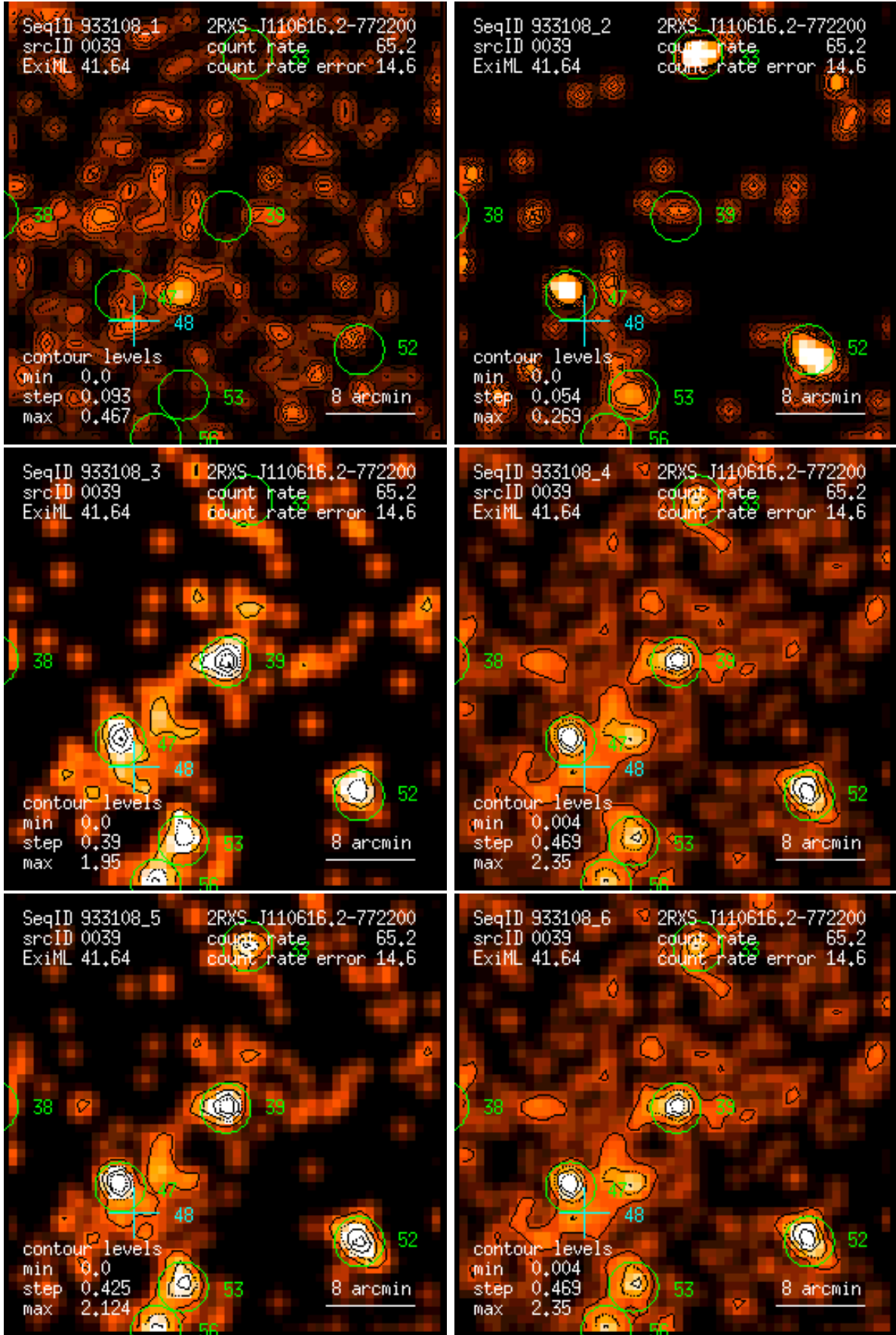
Figure 39: RASS 933108: detection 0039: band rate images, Gaussian filter: (1) PSPC channels 11 – 41, (2) 52 – 90, (3) 91 – 201, (4) 11 – 235, (5) 52 – 201, (6) 11 – 201. Broad band rates in counts/ks. Band rate contour levels in counts/ks/arcmin 2 .
