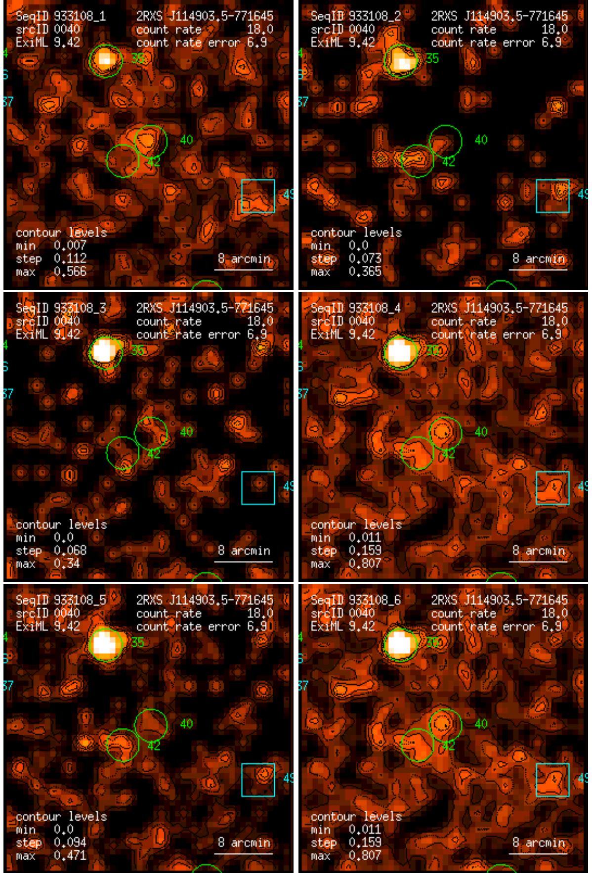
Figure 40: RASS 933108: detection 0040: band rate images, Gaussian filter: (1) PSPC channels 11 – 41, (2) 52 – 90, (3) 91 – 201, (4) 11 – 235, (5) 52 – 201, (6) 11 – 201. Broad band rates in counts/ks. Band rate contour levels in counts/ks/arcmin 2 .
