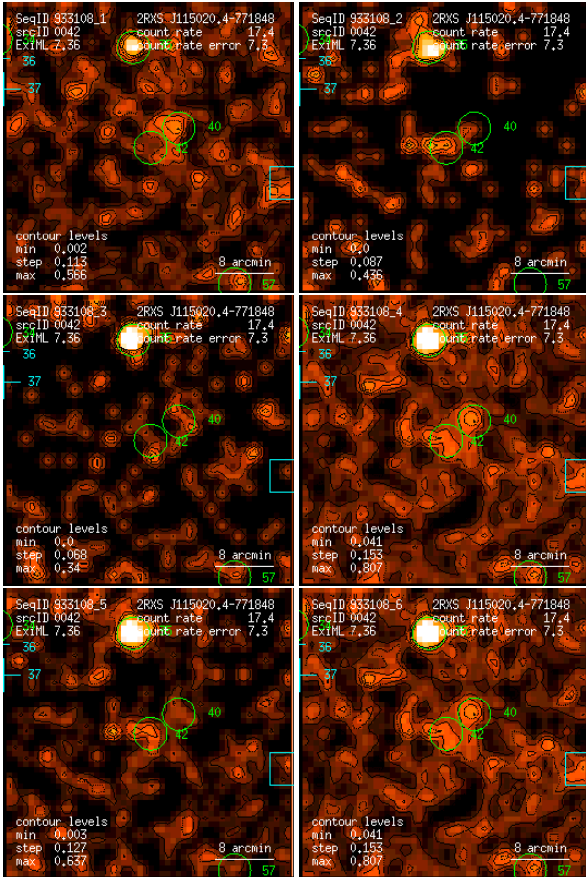
Figure 42: RASS 933108: detection 0042: band rate images, Gaussian filter: (1) PSPC channels 11 – 41, (2) 52 – 90, (3) 91 – 201, (4) 11 – 235, (5) 52 – 201, (6) 11 – 201. Broad band rates in counts/ks. Band rate contour levels in counts/ks/arcmin 2 .
