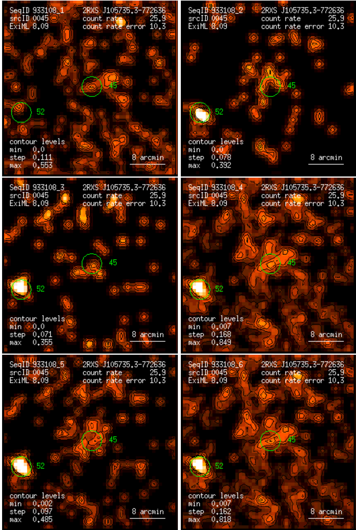
Figure 45: RASS 933108: detection 0045: band rate images, Gaussian filter: (1) PSPC channels 11 – 41, (2) 52 – 90, (3) 91 – 201, (4) 11 – 235, (5) 52 – 201, (6) 11 – 201. Broad band rates in counts/ks. Band rate contour levels in counts/ks/arcmin 2 .
