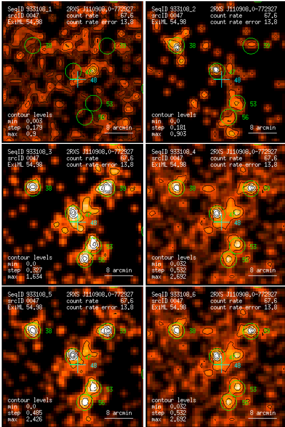
Figure 47: RASS 933108: detection 0047: band rate images, Gaussian filter: (1) PSPC channels 11 – 41, (2) 52 – 90, (3) 91 – 201, (4) 11 – 235, (5) 52 – 201, (6) 11 – 201. Broad band rates in counts/ks. Band rate contour levels in counts/ks/arcmin 2 .
