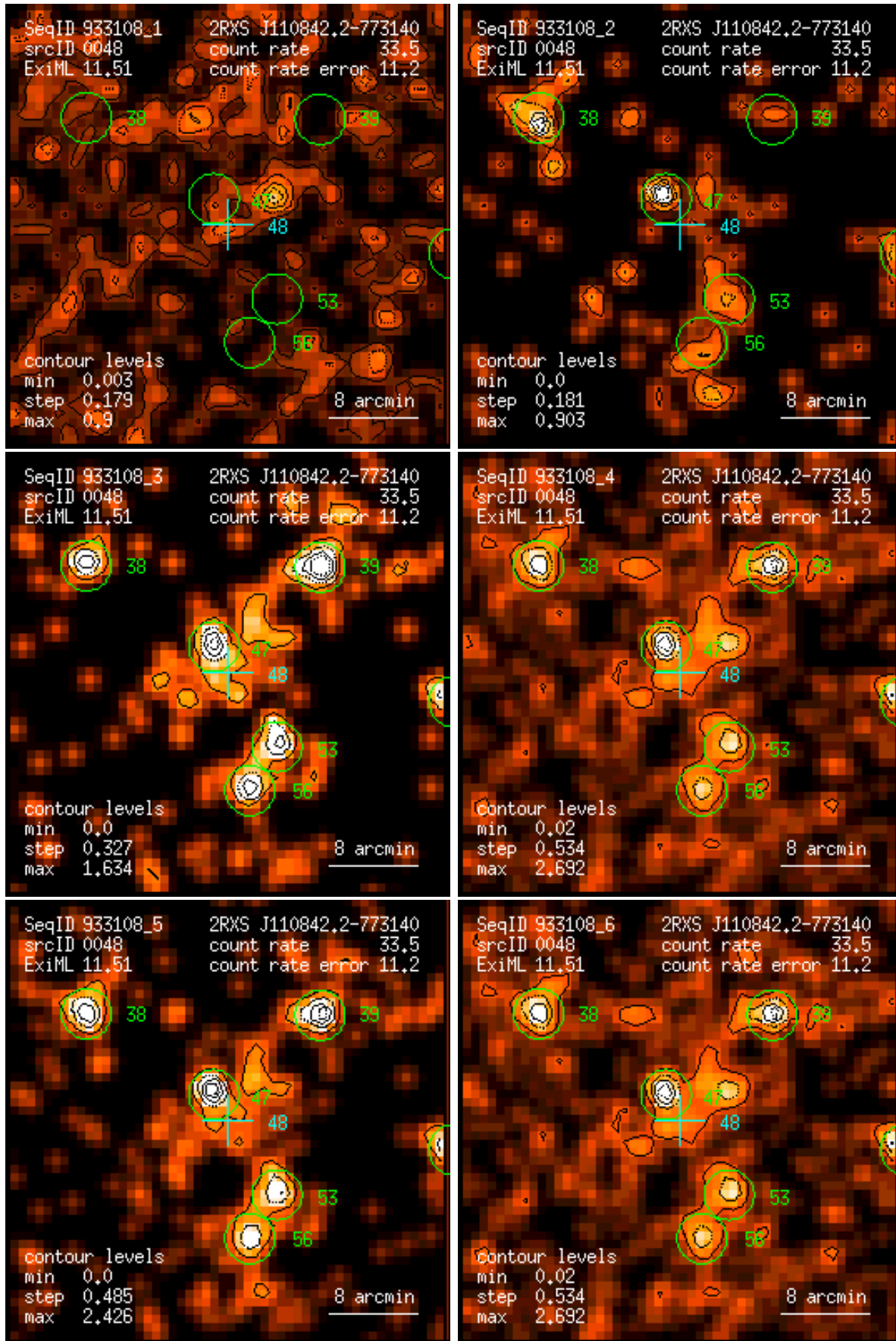
Figure 48: RASS 933108: detection 0048: band rate images, Gaussian filter: (1) PSPC channels 11 – 41, (2) 52 – 90, (3) 91 – 201, (4) 11 – 235, (5) 52 – 201, (6) 11 – 201. Broad band rates in counts/ks. Band rate contour levels in counts/ks/arcmin 2 .
