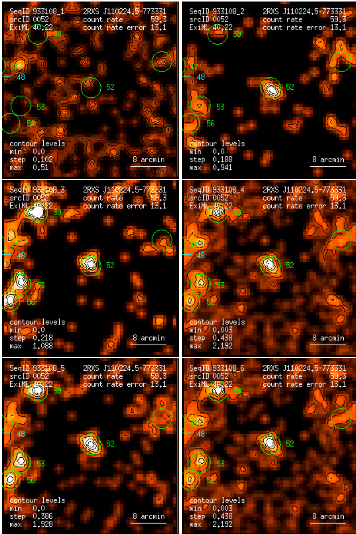
Figure 52: RASS 933108: detection 0052: band rate images, Gaussian filter: (1) PSPC channels 11 – 41, (2) 52 – 90, (3) 91 – 201, (4) 11 – 235, (5) 52 – 201, (6) 11 – 201. Broad band rates in counts/ks. Band rate contour levels in counts/ks/arcmin 2 .
