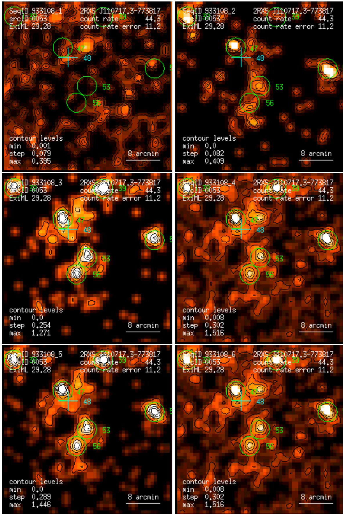
Figure 53: RASS 933108: detection 0053: band rate images, Gaussian filter: (1) PSPC channels 11 – 41, (2) 52 – 90, (3) 91 – 201, (4) 11 – 235, (5) 52 – 201, (6) 11 – 201. Broad band rates in counts/ks. Band rate contour levels in counts/ks/arcmin 2 .
