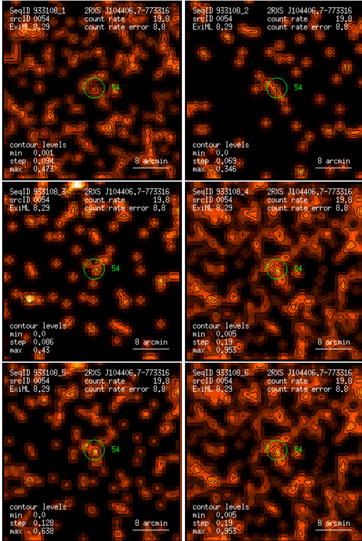
Figure 54: RASS 933108: detection 0054: band rate images, Gaussian filter: (1) PSPC channels 11 – 41, (2) 52 – 90, (3) 91 – 201, (4) 11 – 235, (5) 52 – 201, (6) 11 – 201. Broad band rates in counts/ks. Band rate contour levels in counts/ks/arcmin 2 .
