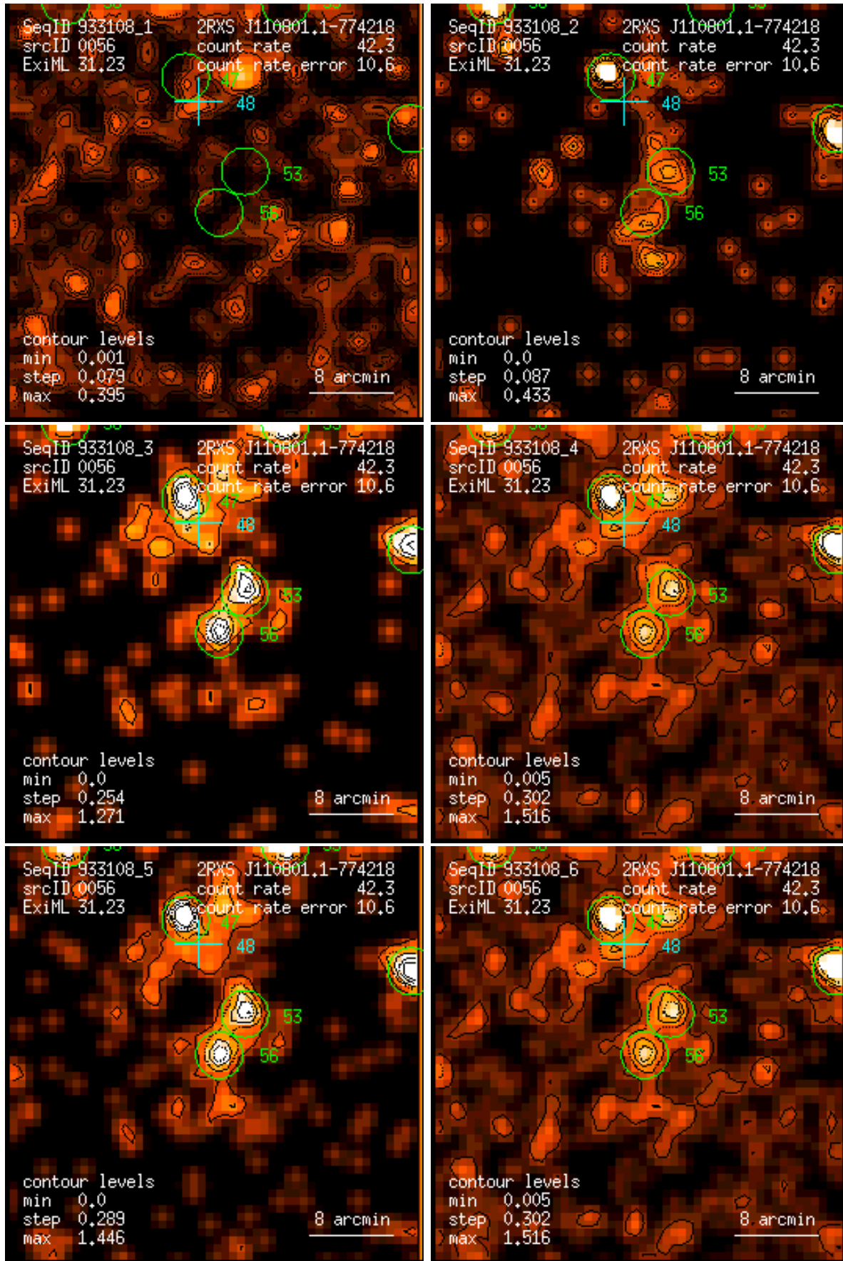
Figure 56: RASS 933108: detection 0056: band rate images, Gaussian filter: (1) PSPC channels 11 – 41, (2) 52 – 90, (3) 91 – 201, (4) 11 – 235, (5) 52 – 201, (6) 11 – 201. Broad band rates in counts/ks. Band rate contour levels in counts/ks/arcmin 2 .
