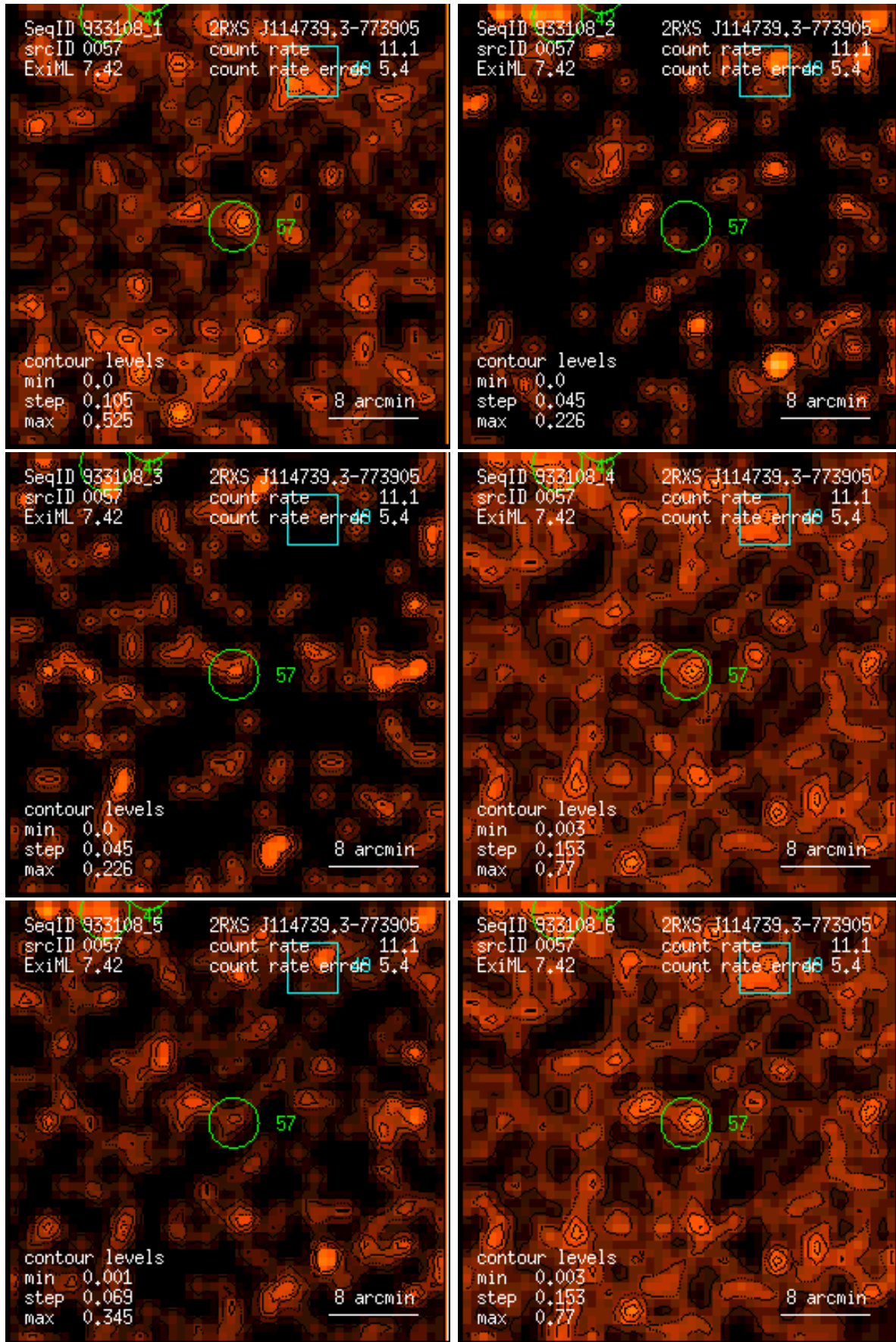
Figure 57: RASS 933108: detection 0057: band rate images, Gaussian filter: (1) PSPC channels 11 – 41, (2) 52 – 90, (3) 91 – 201, (4) 11 – 235, (5) 52 – 201, (6) 11 – 201. Broad band rates in counts/ks. Band rate contour levels in counts/ks/arcmin 2 .
