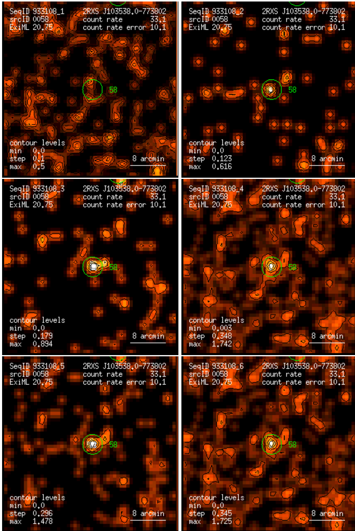
Figure 58: RASS 933108: detection 0058: band rate images, Gaussian filter: (1) PSPC channels 11 – 41, (2) 52 – 90, (3) 91 – 201, (4) 11 – 235, (5) 52 – 201, (6) 11 – 201. Broad band rates in counts/ks. Band rate contour levels in counts/ks/arcmin 2 .
