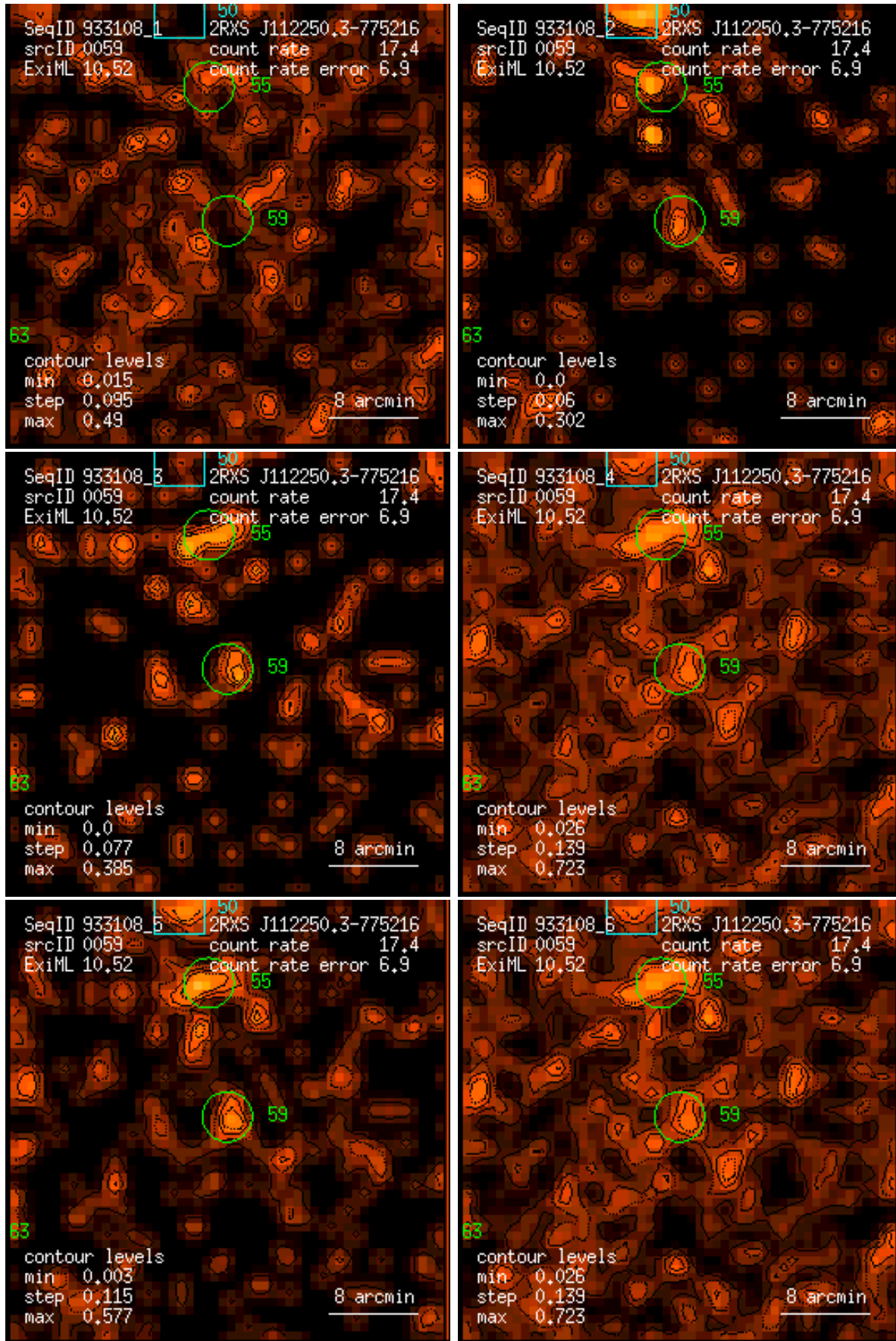
Figure 59: RASS 933108: detection 0059: band rate images, Gaussian filter: (1) PSPC channels 11 – 41, (2) 52 – 90, (3) 91 – 201, (4) 11 – 235, (5) 52 – 201, (6) 11 – 201. Broad band rates in counts/ks. Band rate contour levels in counts/ks/arcmin 2 .
