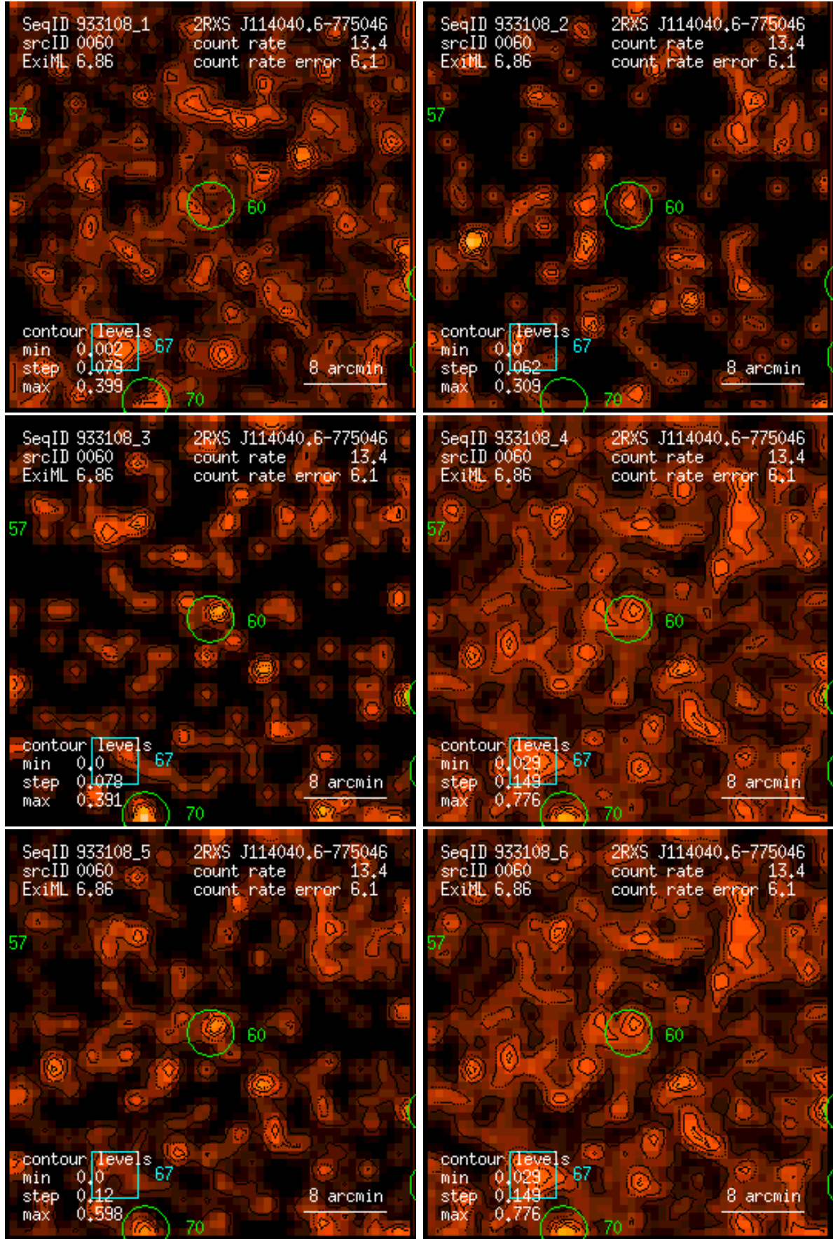
Figure 60: RASS 933108: detection 0060: band rate images, Gaussian filter: (1) PSPC channels 11 – 41, (2) 52 – 90, (3) 91 – 201, (4) 11 – 235, (5) 52 – 201, (6) 11 – 201. Broad band rates in counts/ks. Band rate contour levels in counts/ks/arcmin 2 .
