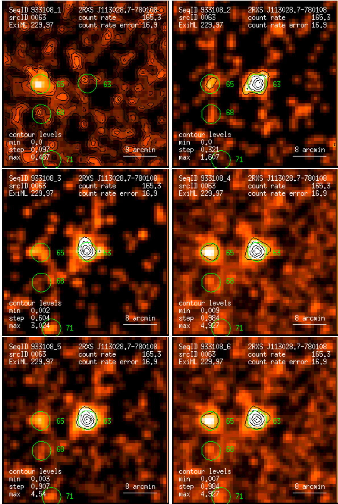
Figure 63: RASS 933108: detection 0063: band rate images, Gaussian filter: (1) PSPC channels 11 – 41, (2) 52 – 90, (3) 91 – 201, (4) 11 – 235, (5) 52 – 201, (6) 11 – 201. Broad band rates in counts/ks. Band rate contour levels in counts/ks/arcmin 2 .
