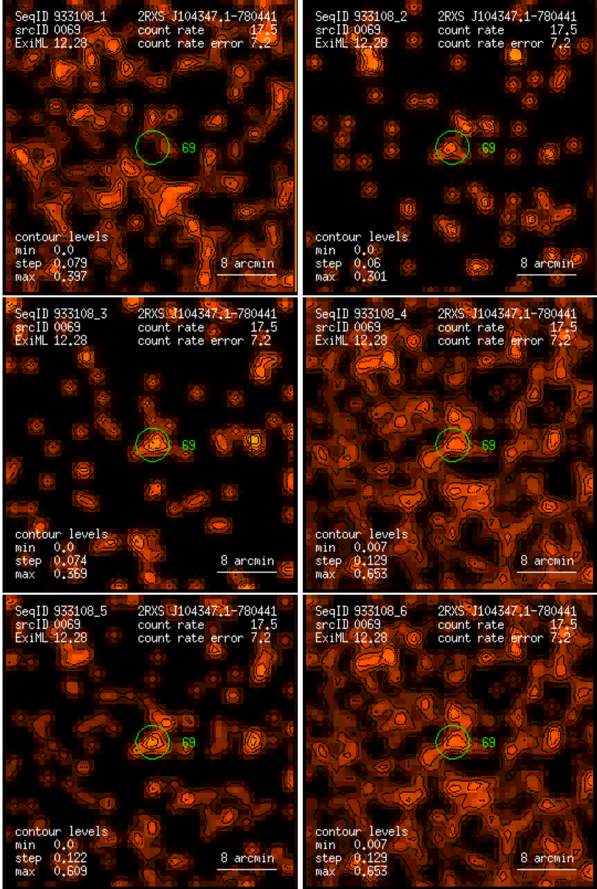
Figure 69: RASS 933108: detection 0069: band rate images, Gaussian filter: (1) PSPC channels 11 – 41, (2) 52 – 90, (3) 91 – 201, (4) 11 – 235, (5) 52 – 201, (6) 11 – 201. Broad band rates in counts/ks. Band rate contour levels in counts/ks/arcmin 2 .
