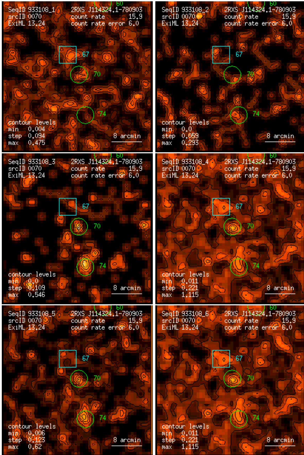
Figure 70: RASS 933108: detection 0070: band rate images, Gaussian filter: (1) PSPC channels 11 – 41, (2) 52 – 90, (3) 91 – 201, (4) 11 – 235, (5) 52 – 201, (6) 11 – 201. Broad band rates in counts/ks. Band rate contour levels in counts/ks/arcmin 2 .
