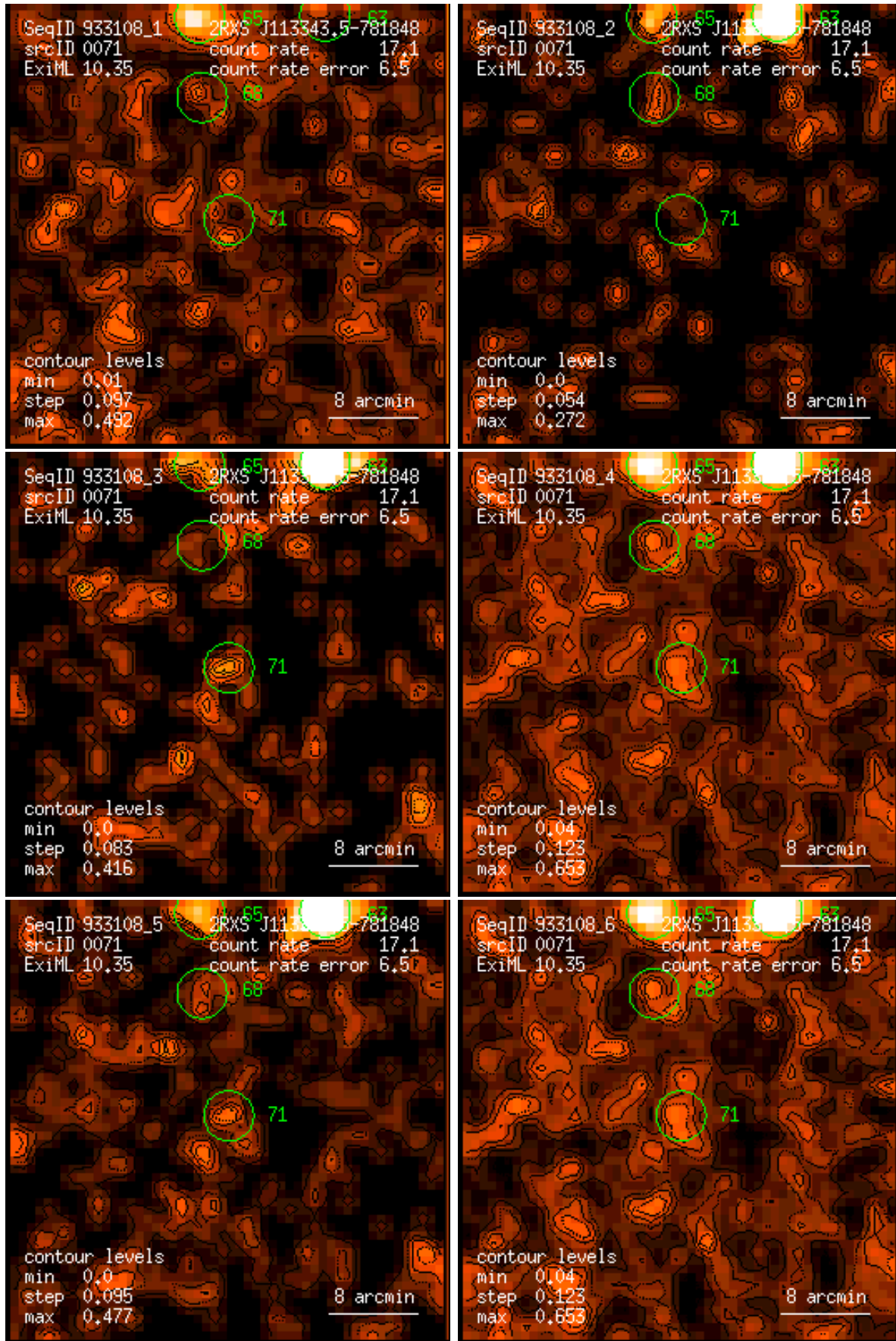
Figure 71: RASS 933108: detection 0071: band rate images, Gaussian filter: (1) PSPC channels 11 – 41, (2) 52 – 90, (3) 91 – 201, (4) 11 – 235, (5) 52 – 201, (6) 11 – 201. Broad band rates in counts/ks. Band rate contour levels in counts/ks/arcmin 2 .
