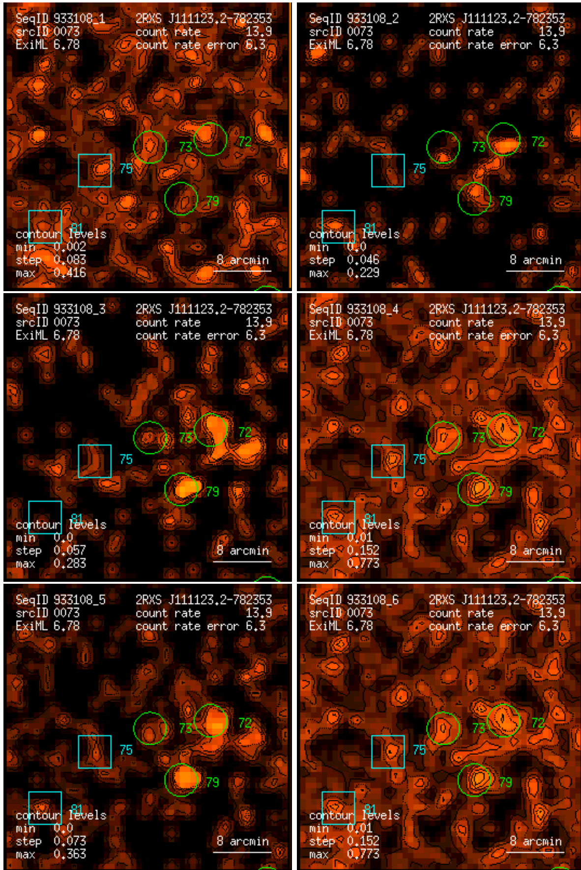
Figure 73: RASS 933108: detection 0073: band rate images, Gaussian filter: (1) PSPC channels 11 – 41, (2) 52 – 90, (3) 91 – 201, (4) 11 – 235, (5) 52 – 201, (6) 11 – 201. Broad band rates in counts/ks. Band rate contour levels in counts/ks/arcmin 2 .
