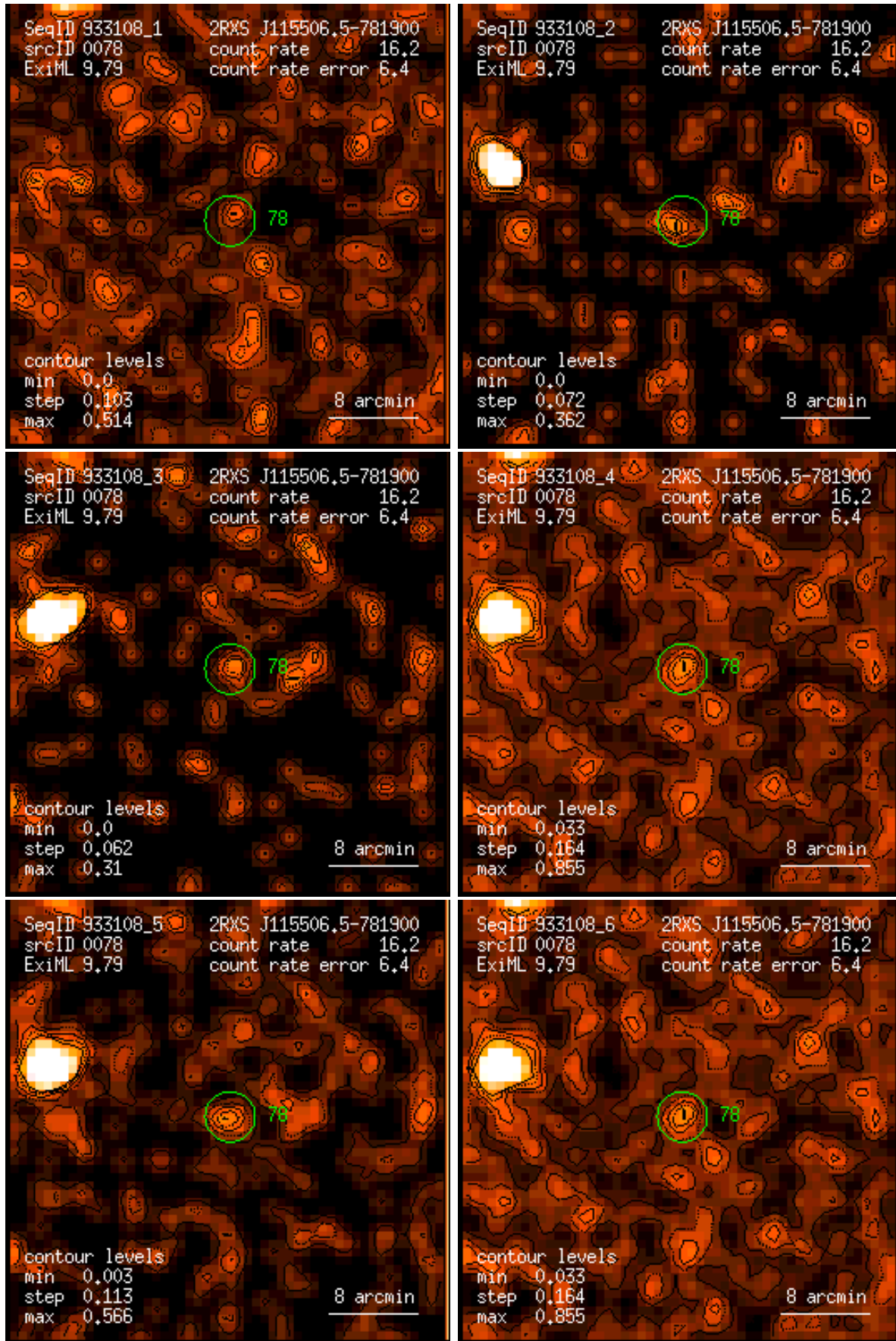
Figure 78: RASS 933108: detection 0078: band rate images, Gaussian filter: (1) PSPC channels 11 – 41, (2) 52 – 90, (3) 91 – 201, (4) 11 – 235, (5) 52 – 201, (6) 11 – 201. Broad band rates in counts/ks. Band rate contour levels in counts/ks/arcmin 2 .
