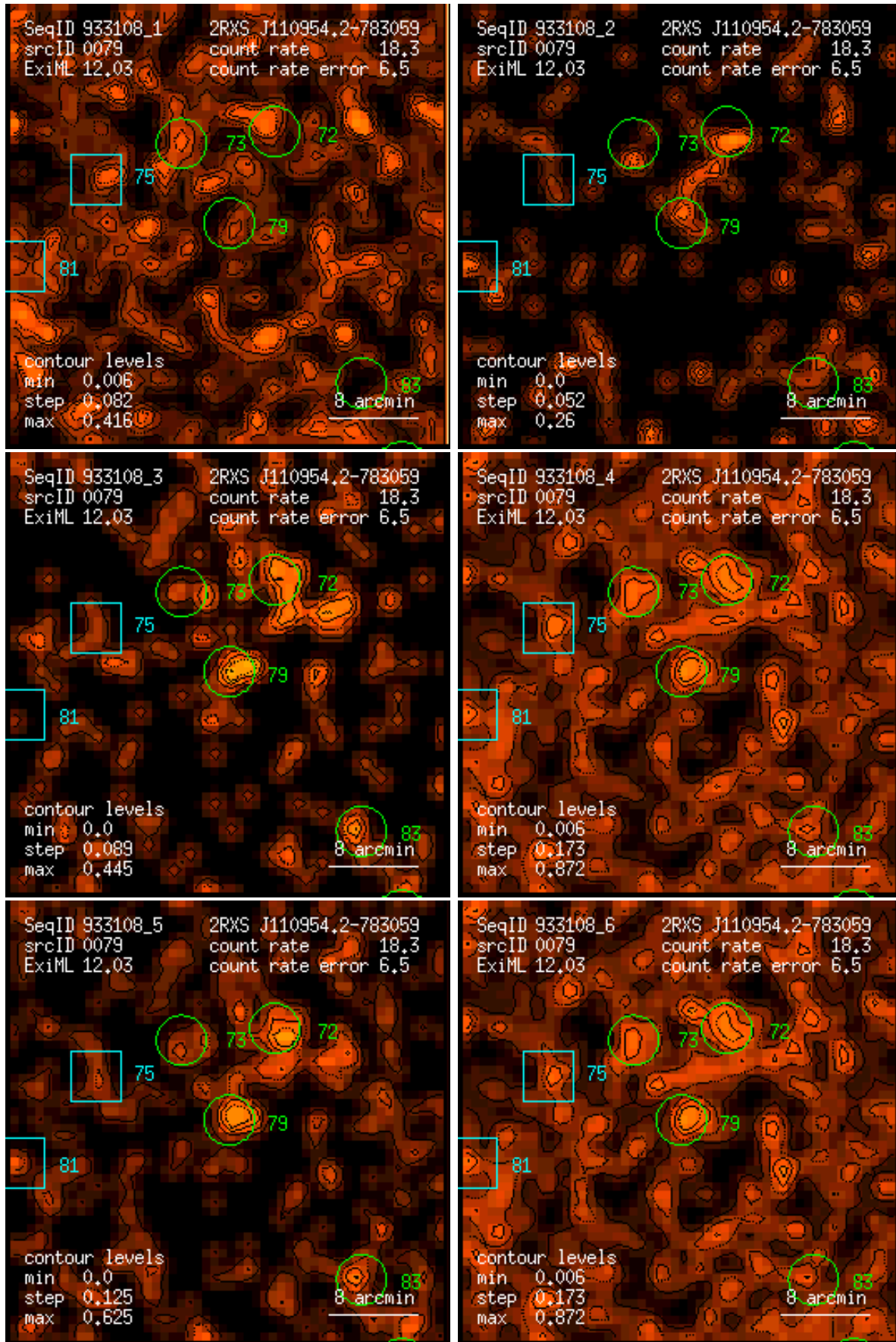
Figure 79: RASS 933108: detection 0079: band rate images, Gaussian filter: (1) PSPC channels 11 – 41, (2) 52 – 90, (3) 91 – 201, (4) 11 – 235, (5) 52 – 201, (6) 11 – 201. Broad band rates in counts/ks. Band rate contour levels in counts/ks/arcmin 2 .
