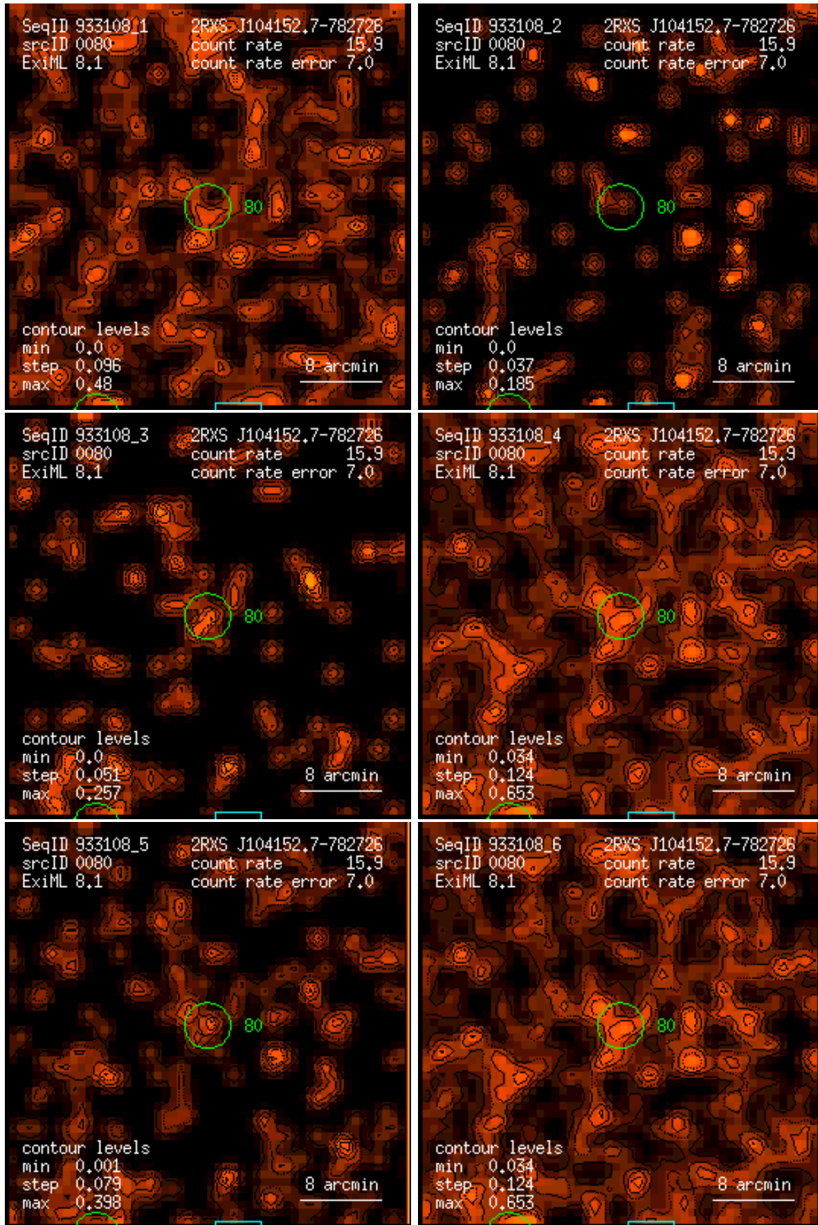
Figure 80: RASS 933108: detection 0080: band rate images, Gaussian filter: (1) PSPC channels 11 – 41, (2) 52 – 90, (3) 91 – 201, (4) 11 – 235, (5) 52 – 201, (6) 11 – 201. Broad band rates in counts/ks. Band rate contour levels in counts/ks/arcmin 2 .
