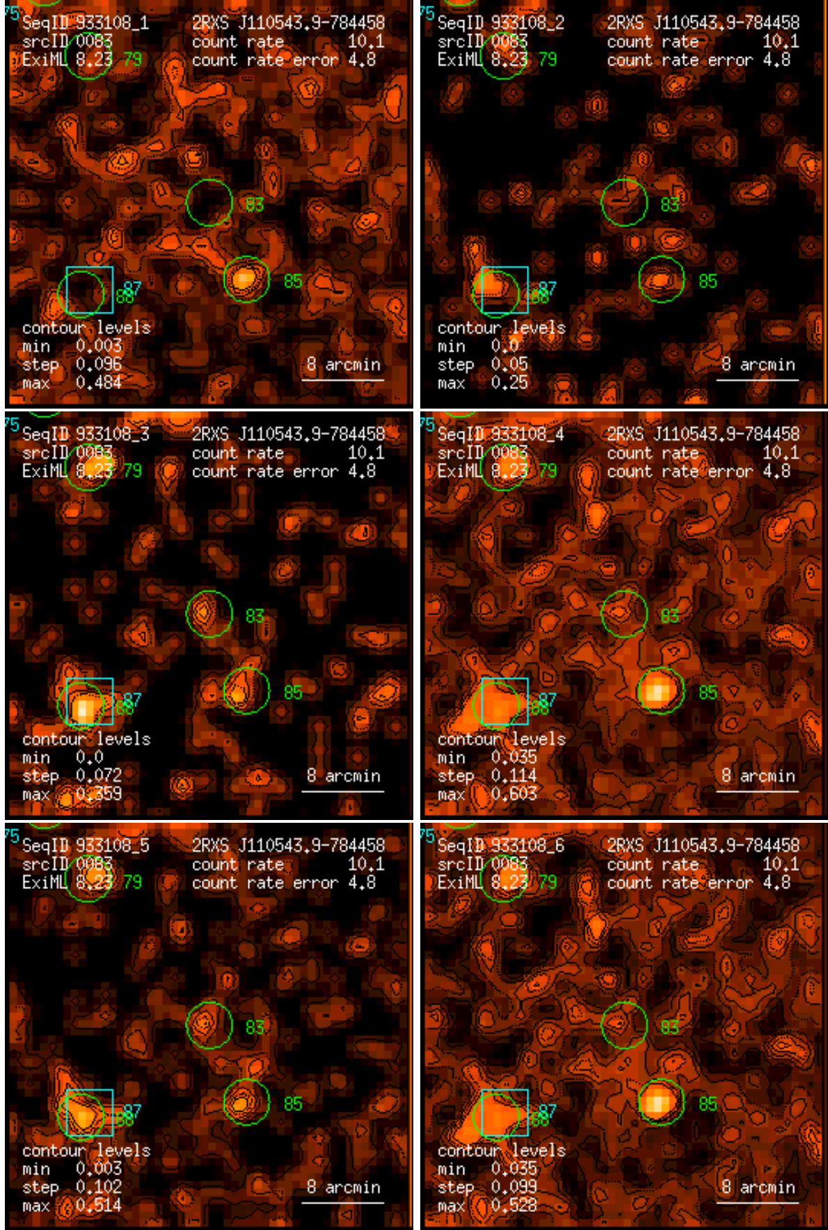
Figure 83: RASS 933108: detection 0083: band rate images, Gaussian filter: (1) PSPC channels 11 – 41, (2) 52 – 90, (3) 91 – 201, (4) 11 – 235, (5) 52 – 201, (6) 11 – 201. Broad band rates in counts/ks. Band rate contour levels in counts/ks/arcmin 2 .
