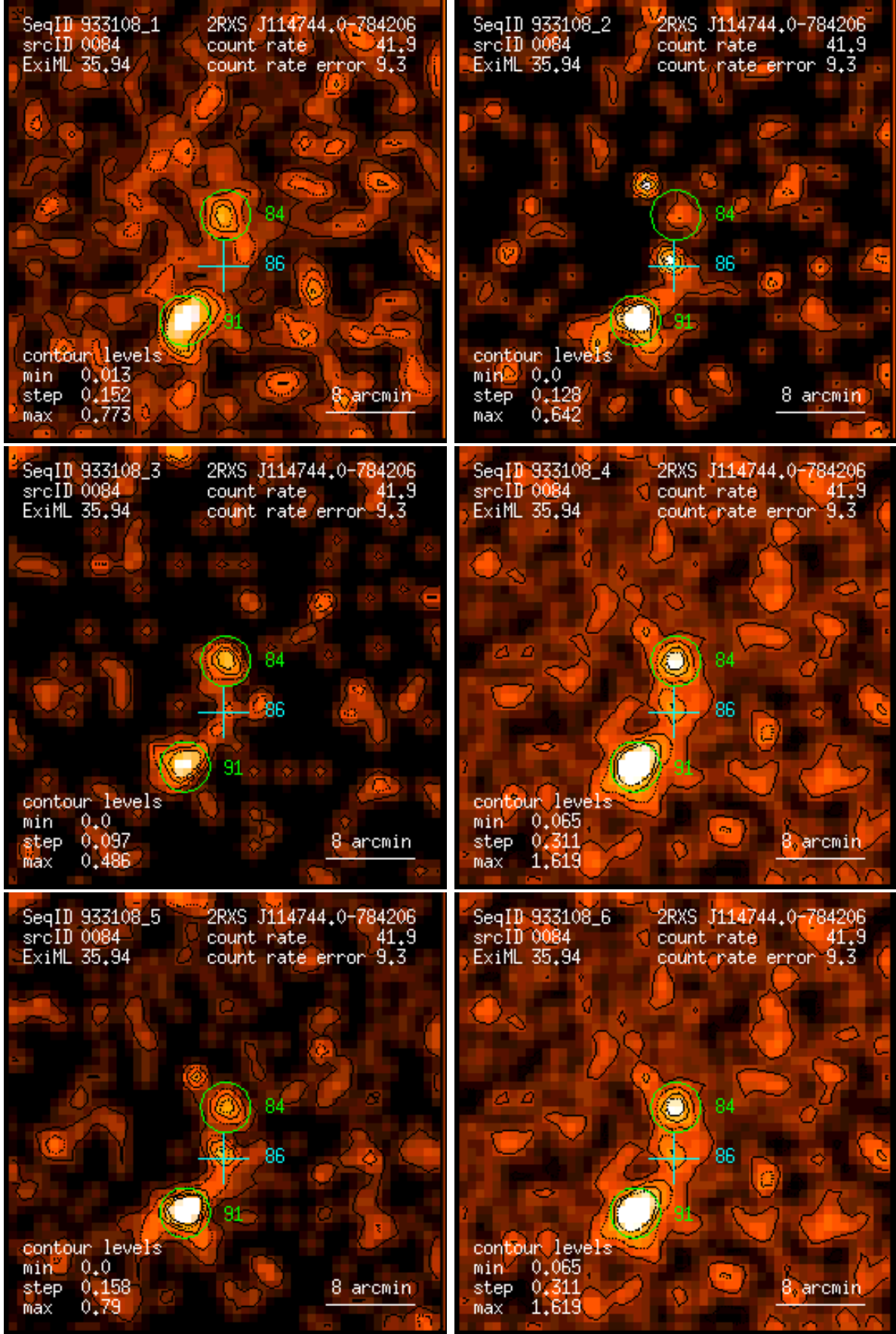
Figure 84: RASS 933108: detection 0084: band rate images, Gaussian filter: (1) PSPC channels 11 – 41, (2) 52 – 90, (3) 91 – 201, (4) 11 – 235, (5) 52 – 201, (6) 11 – 201. Broad band rates in counts/ks. Band rate contour levels in counts/ks/arcmin 2 .
