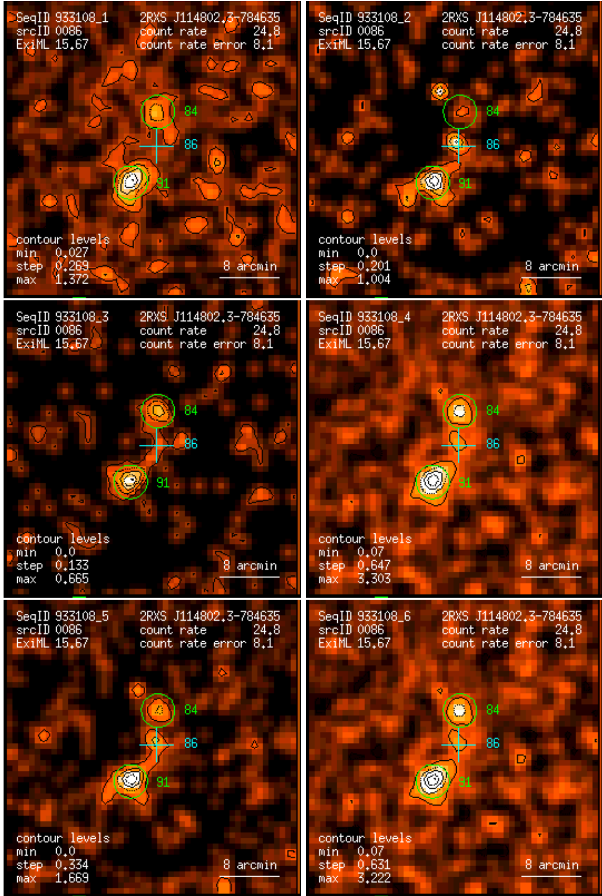
Figure 86: RASS 933108: detection 0086: band rate images, Gaussian filter: (1) PSPC channels 11 – 41, (2) 52 – 90, (3) 91 – 201, (4) 11 – 235, (5) 52 – 201, (6) 11 – 201. Broad band rates in counts/ks. Band rate contour levels in counts/ks/arcmin 2 .
