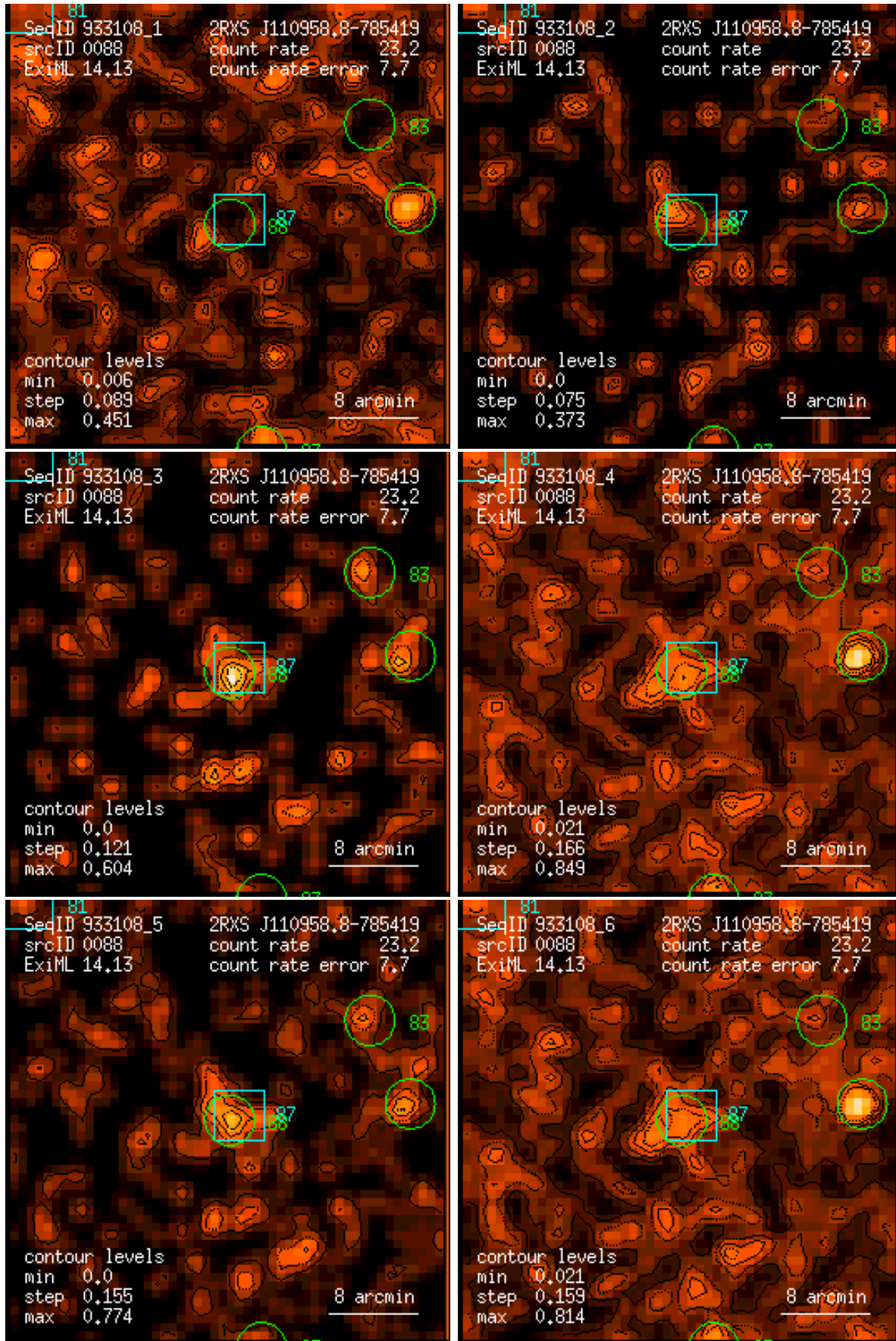
Figure 88: RASS 933108: detection 0088: band rate images, Gaussian filter: (1) PSPC channels 11 – 41, (2) 52 – 90, (3) 91 – 201, (4) 11 – 235, (5) 52 – 201, (6) 11 – 201. Broad band rates in counts/ks. Band rate contour levels in counts/ks/arcmin 2 .
