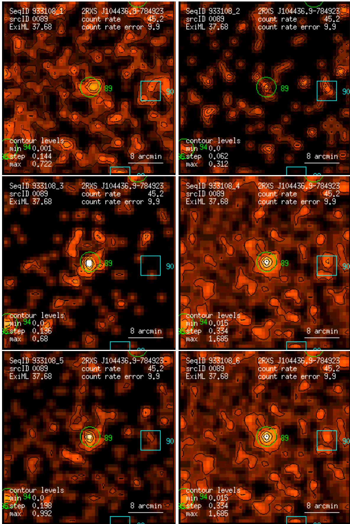
Figure 89: RASS 933108: detection 0089: band rate images, Gaussian filter: (1) PSPC channels 11 – 41, (2) 52 – 90, (3) 91 – 201, (4) 11 – 235, (5) 52 – 201, (6) 11 – 201. Broad band rates in counts/ks. Band rate contour levels in counts/ks/arcmin 2 .
