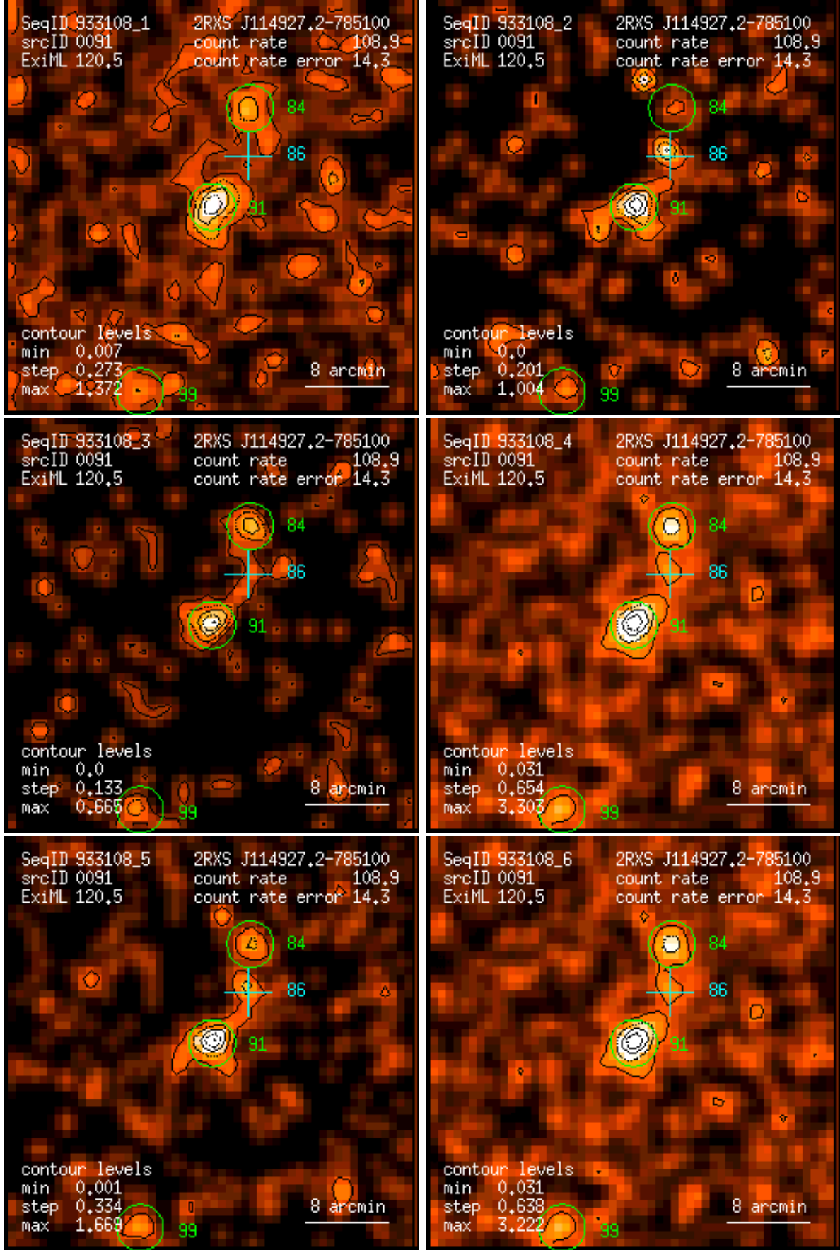
Figure 91: RASS 933108: detection 0091: band rate images, Gaussian filter: (1) PSPC channels 11 – 41, (2) 52 – 90, (3) 91 – 201, (4) 11 – 235, (5) 52 – 201, (6) 11 – 201. Broad band rates in counts/ks. Band rate contour levels in counts/ks/arcmin 2 .
