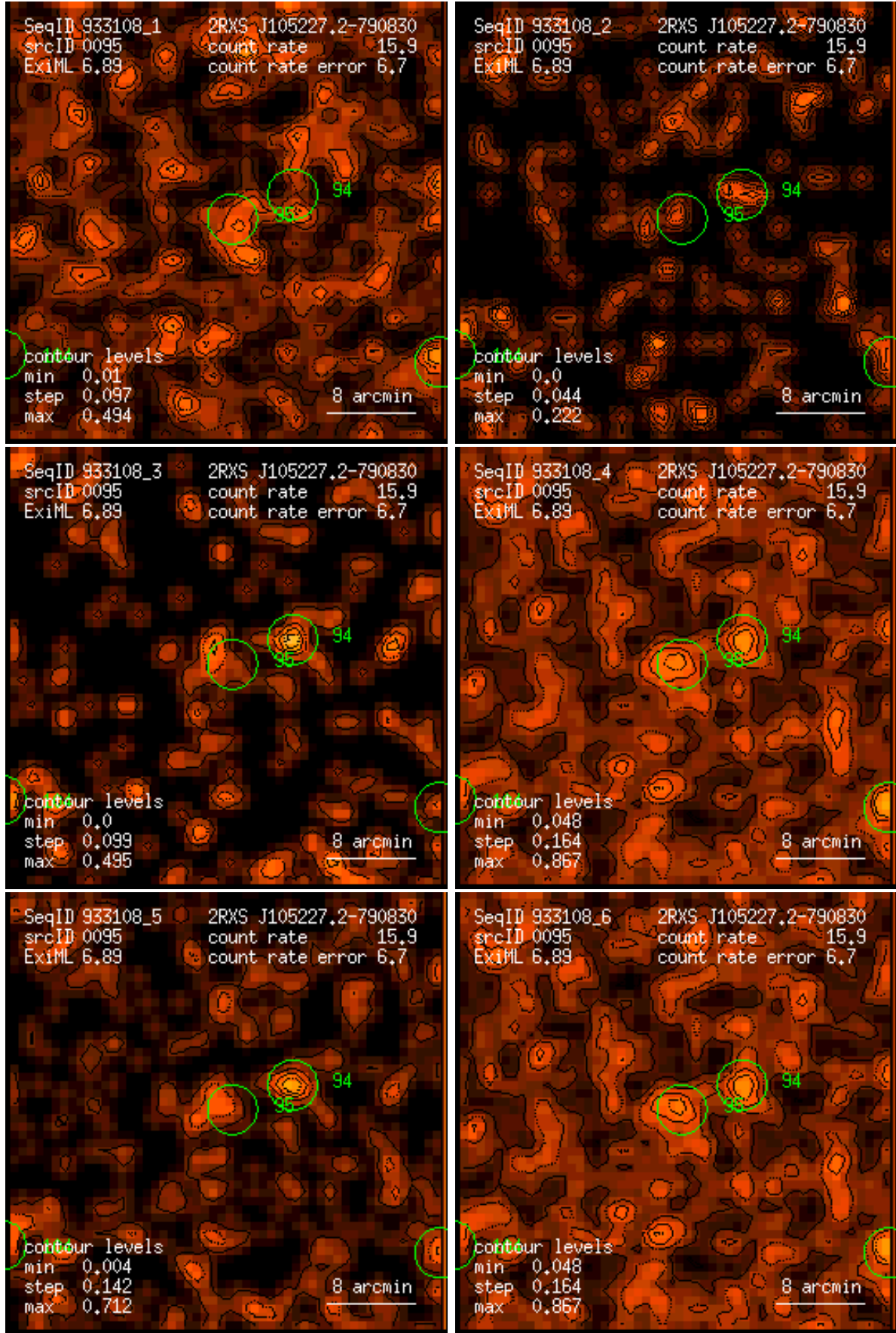
Figure 95: RASS 933108: detection 0095: band rate images, Gaussian filter: (1) PSPC channels 11 – 41, (2) 52 – 90, (3) 91 – 201, (4) 11 – 235, (5) 52 – 201, (6) 11 – 201. Broad band rates in counts/ks. Band rate contour levels in counts/ks/arcmin 2 .
