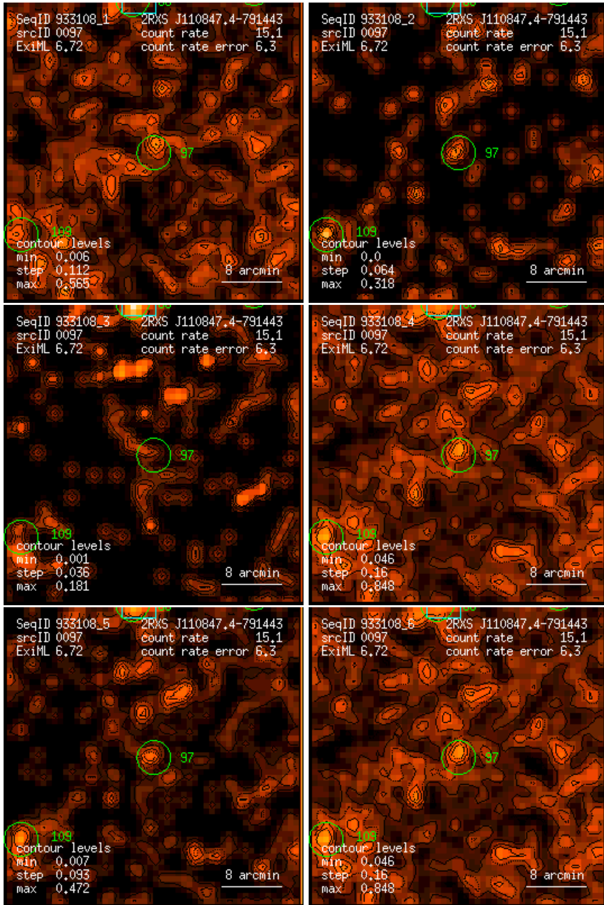
Figure 97: RASS 933108: detection 0097: band rate images, Gaussian filter: (1) PSPC channels 11 – 41, (2) 52 – 90, (3) 91 – 201, (4) 11 – 235, (5) 52 – 201, (6) 11 – 201. Broad band rates in counts/ks. Band rate contour levels in counts/ks/arcmin 2 .
