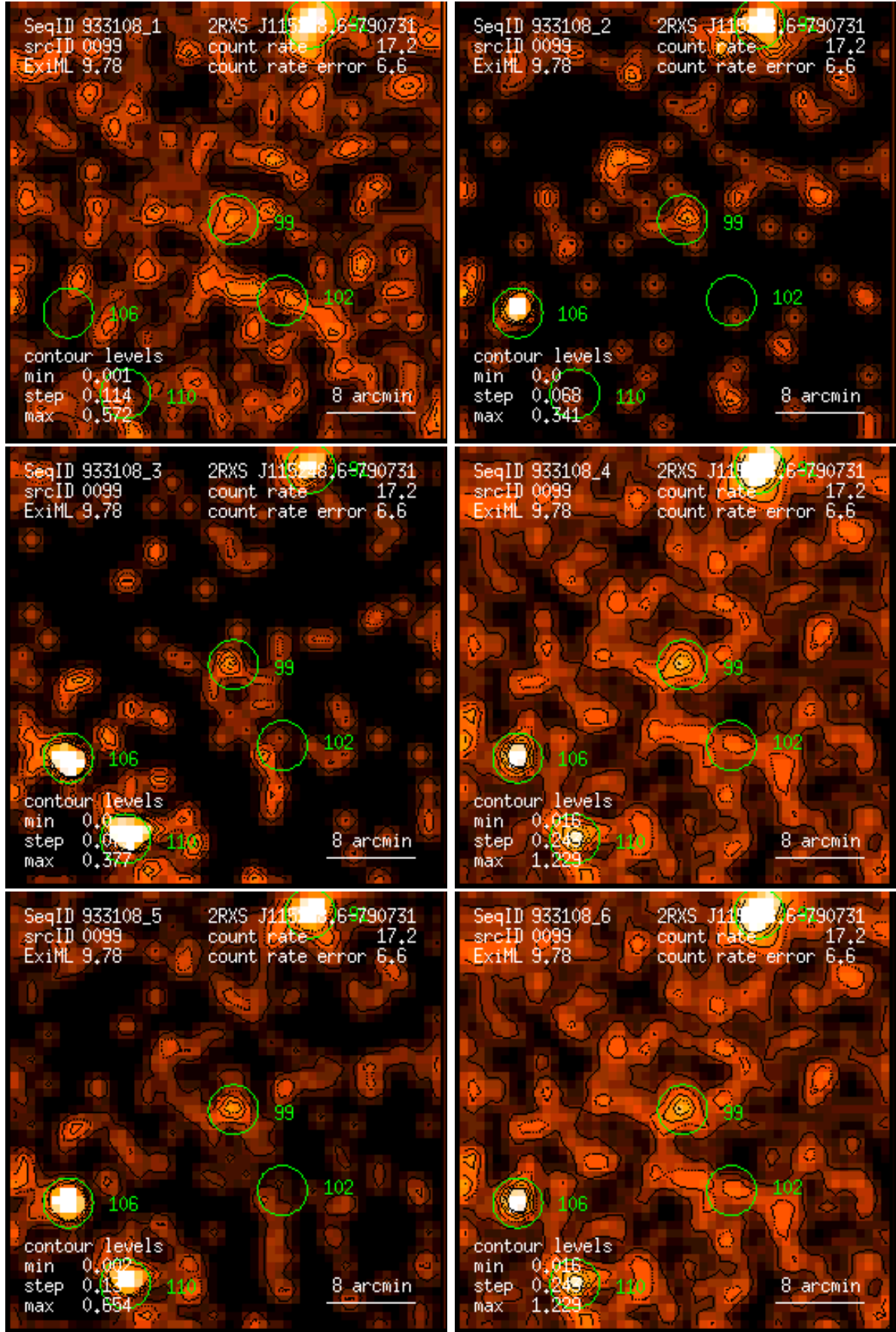
Figure 99: RASS 933108: detection 0099: band rate images, Gaussian filter: (1) PSPC channels 11 – 41, (2) 52 – 90, (3) 91 – 201, (4) 11 – 235, (5) 52 – 201, (6) 11 – 201. Broad band rates in counts/ks. Band rate contour levels in counts/ks/arcmin 2 .
