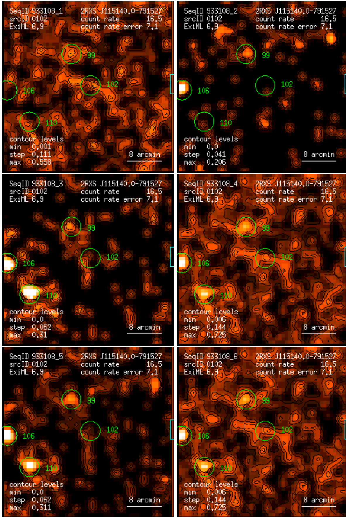
Figure 102: RASS 933108: detection 0102: band rate images, Gaussian filter: (1) PSPC channels 11 – 41, (2) 52 – 90, (3) 91 – 201, (4) 11 – 235, (5) 52 – 201, (6) 11 – 201. Broad band rates in counts/ks. Band rate contour levels in counts/ks/arcmin 2 .
