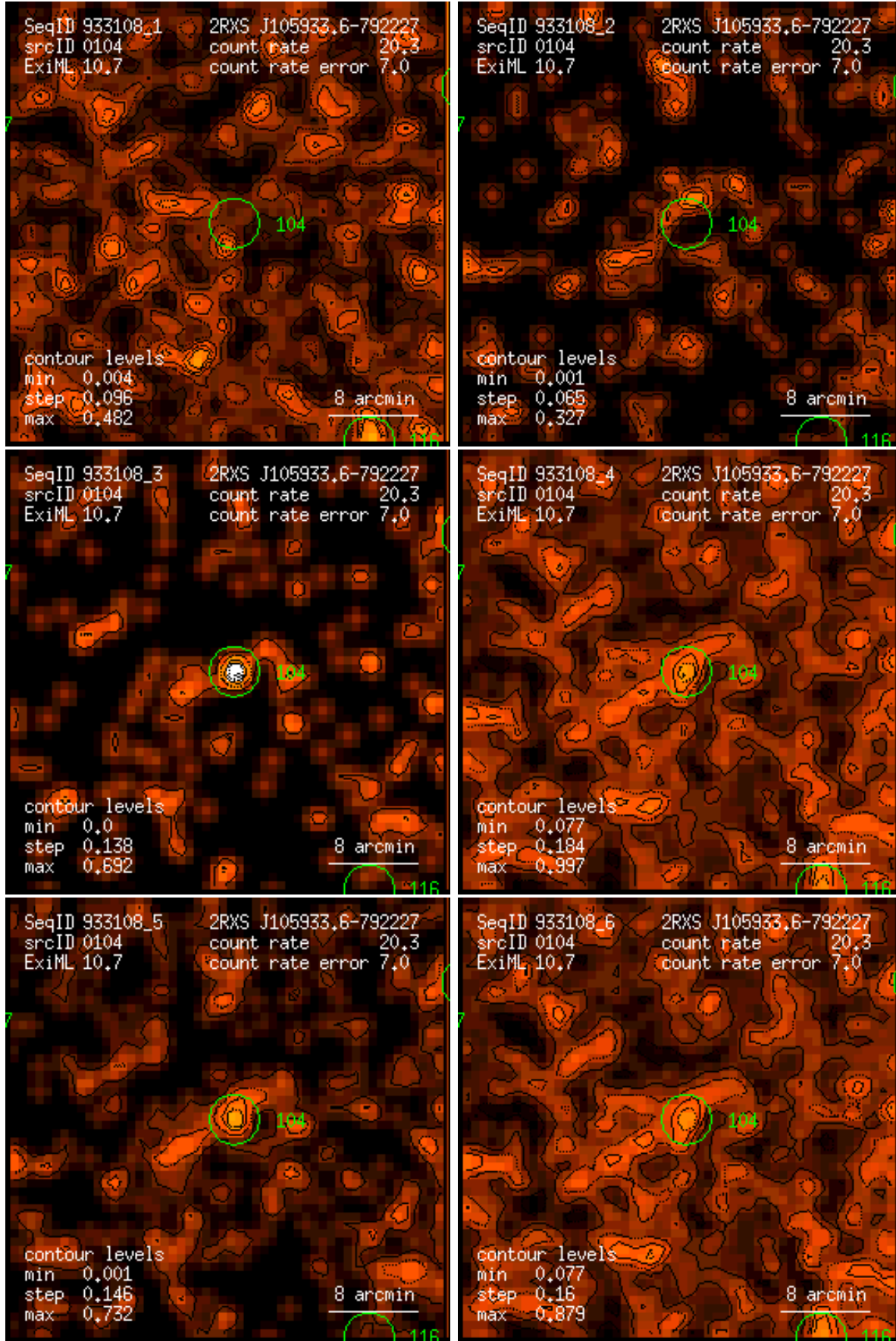
Figure 104: RASS 933108: detection 0104: band rate images, Gaussian filter: (1) PSPC channels 11 – 41, (2) 52 – 90, (3) 91 – 201, (4) 11 – 235, (5) 52 – 201, (6) 11 – 201. Broad band rates in counts/ks. Band rate contour levels in counts/ks/arcmin 2 .
